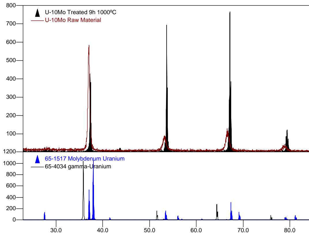
Figure 2. Diffractogram of raw molten U-10Mo and treated at 1000°C during 9h. \text{UMo}_2 and gamma-U are also shown as references.
