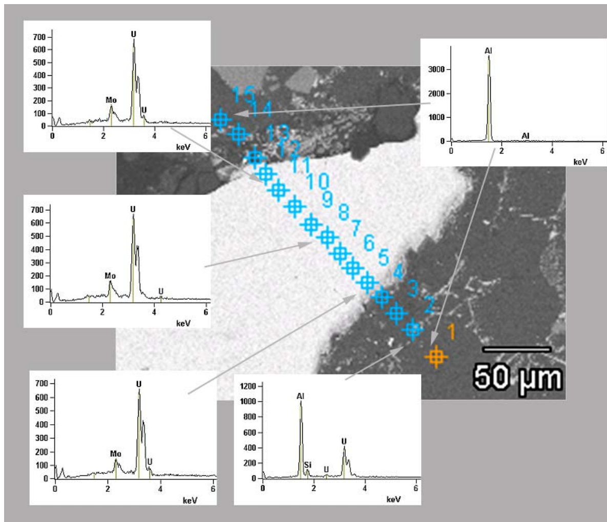
Figure 3. SEM and EDS measurements of U-10Mo surrounded by Al and Al-(U,Mo) subproducts forming the interaction layer. Between the marks 2 and 4 presumably is the region of subproducts in a band around 50μm
