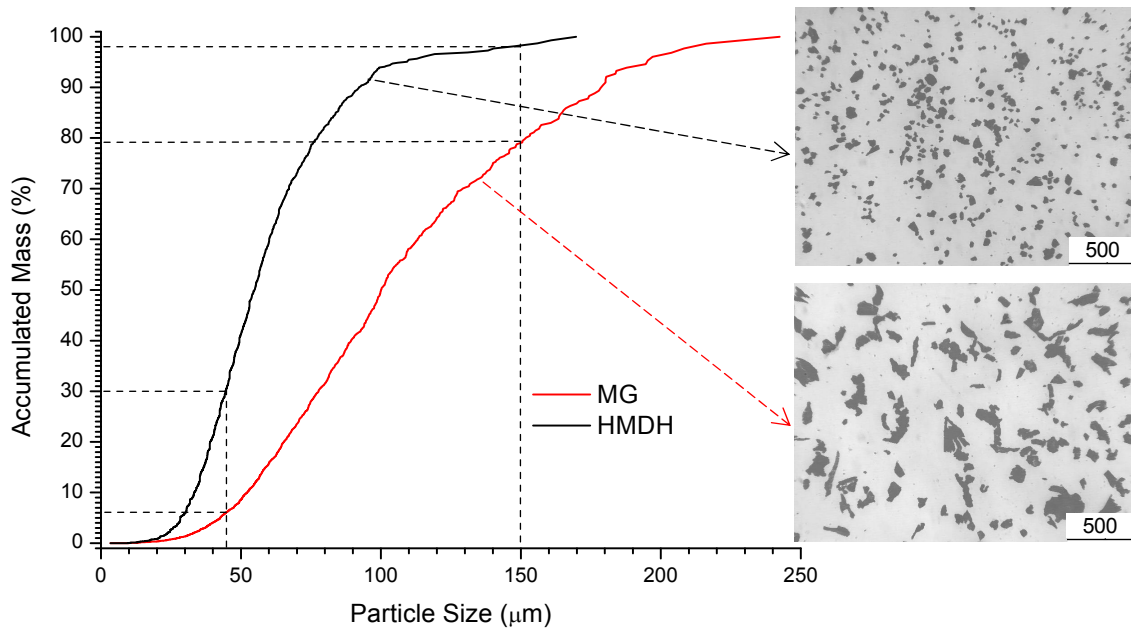
Figure 3 - Particle size distribution curves for the powders prepared by mechanical grinding route (MG – red curve) and hydrogenation-milling-dehydrogenation route (HMDH – black curve).
