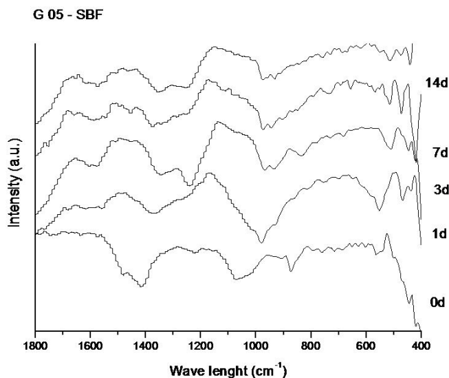
Fig. 4: DRIFT spectra of bioglasses samples after different periods in SBF immersion
