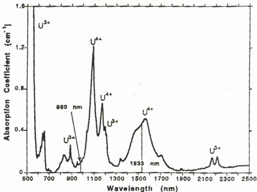
Figure 1. U:SrF 2 absorption spectrum.
