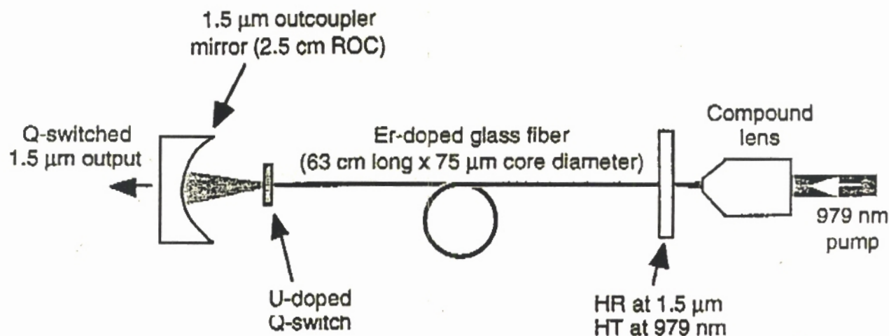
Figure 2. Diagram of Q-switched fiber laser.
