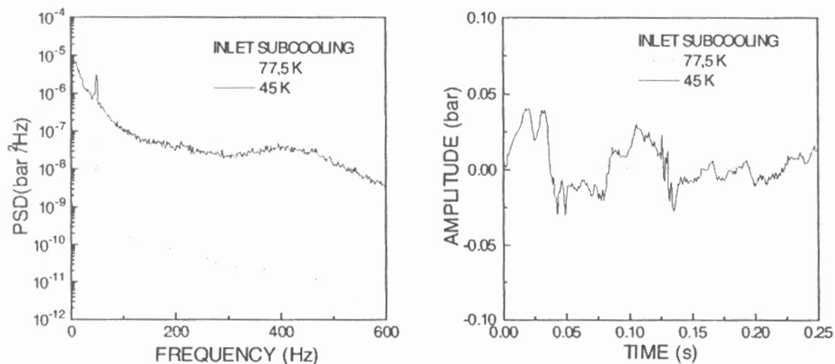
Figure 3. - Pressure Sensor P2X Signal in Frequency and Time Domain - ONB Condition.
