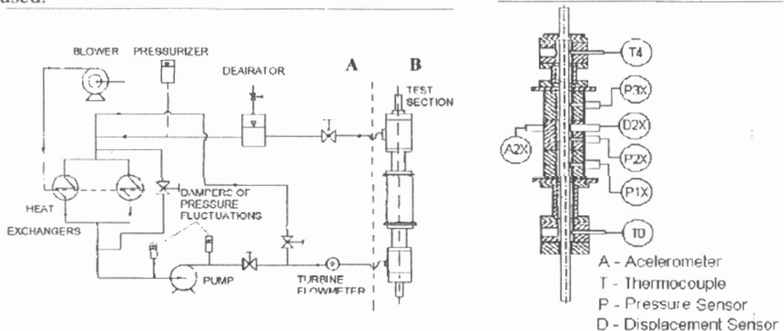
Figure 2. - Experimental Loop for Subcooled Boiling - Flow Diagram and Test Section.
