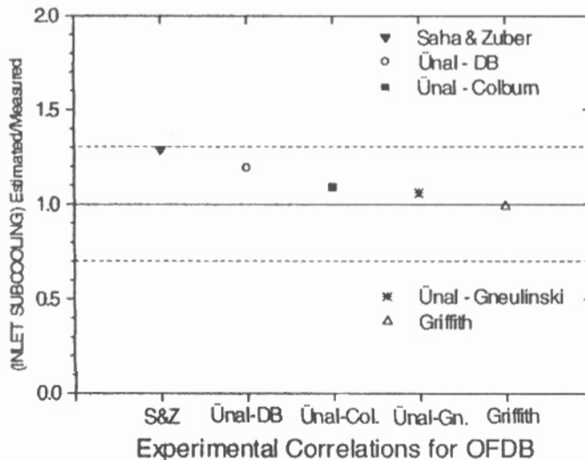
Figure 6 - Estimated to Measured Inlet Subcooling Ratio for the OFDB Condition.
