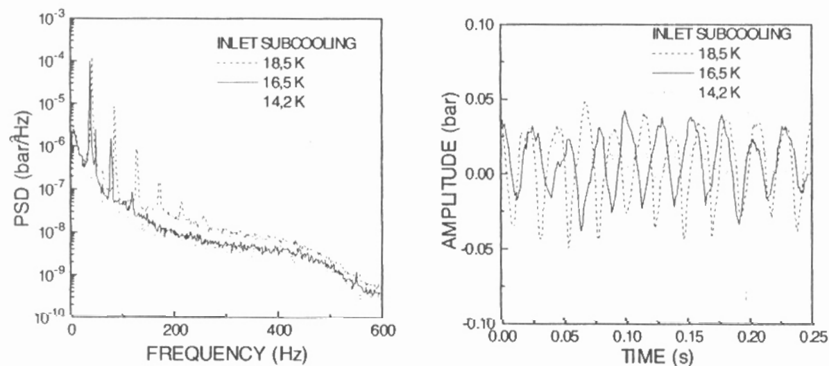
Figure 4. - Pressure Sensor P2X Signal in Frequency and Time Domain. OFDB Condition.
