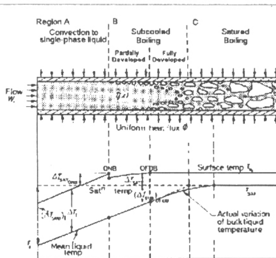
Figure 1 - Schematic Representation of the Subcooled Boiling Regimen.
