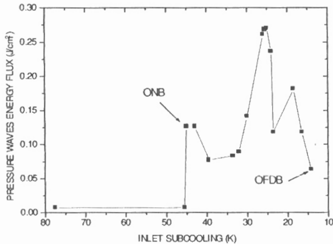
Figure 5. - Pressure Waves Energy Flux Versus Inlet Subcooling in the Pressure Sensor P2X.
