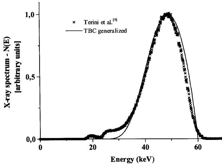
Figure 1 – Comparative results between measurements performed by a Si photodiode operated at room temperature (6) and computer simulation using the waveform generalised TBC model. The experimental conditions are presented in Table 1 for of 60 kVp, and they were the same used for the computer simulation.
