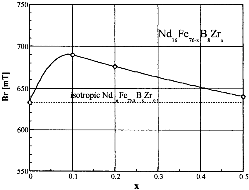
Fig. 1 – Normalised remanence of NdFeBZr magnets.
