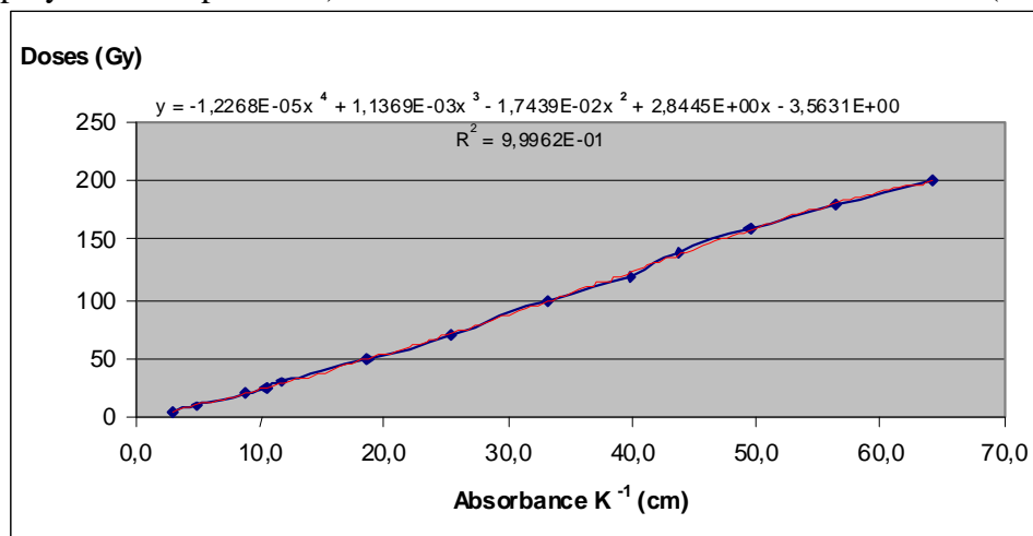
Figure 3. Calibration Curve of the Gafchromic dosimeter
