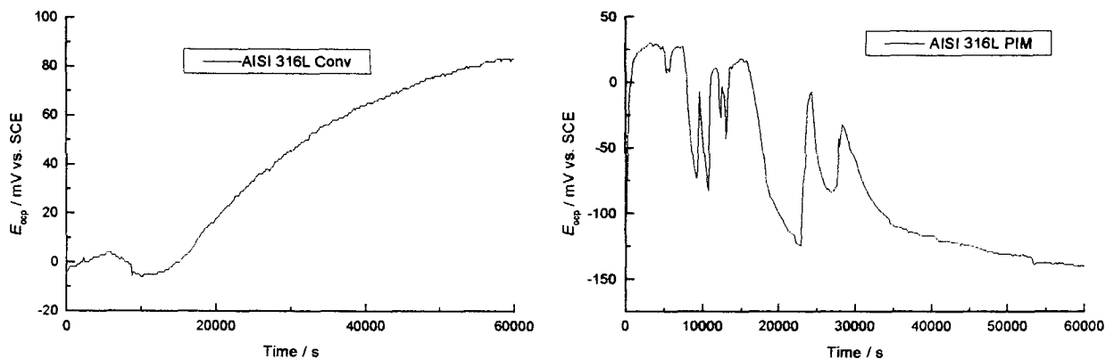
Fig. 1. Open circuit potential variation with time of conventional and PIM 316L steels in MEM.
