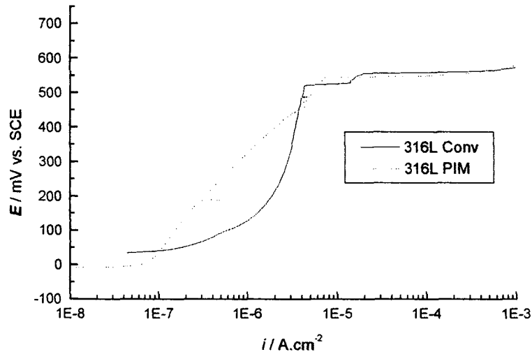
Fig. 2. Potentiodynamic polarization curves of conventional and PIM 316L steels after 10 days immersion in MEM's solution at 37 °C. Scanning rate: 1 mV/s.
