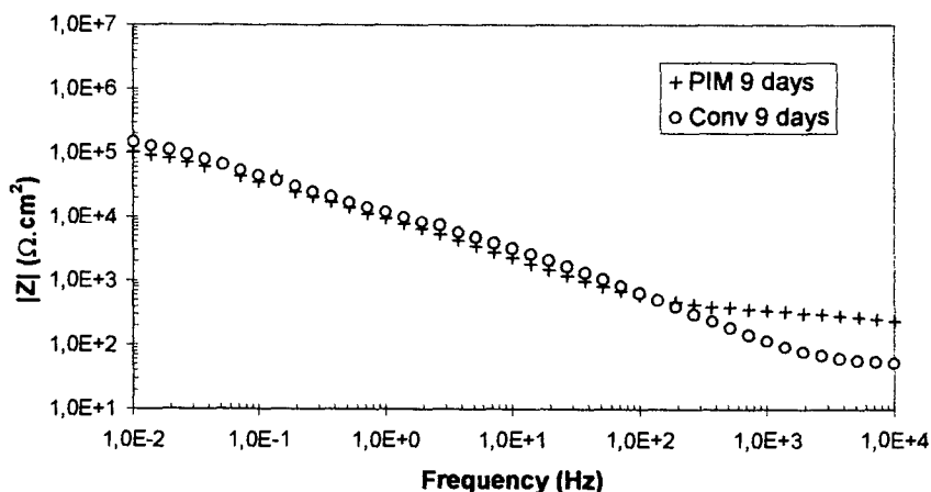
Fig. 5. Bode diagrams for AISI 316L steels, after 9 days of immersion in MEM solution at 37 °C.
