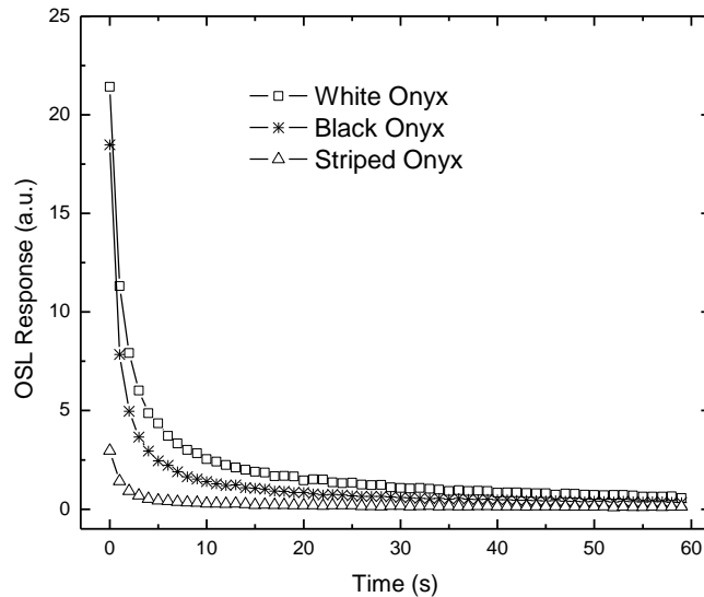
Figure 1. OSL response of Onyx-Teflon pellets irradiated with 5 kGy ( ^{60}\text{Co} )
