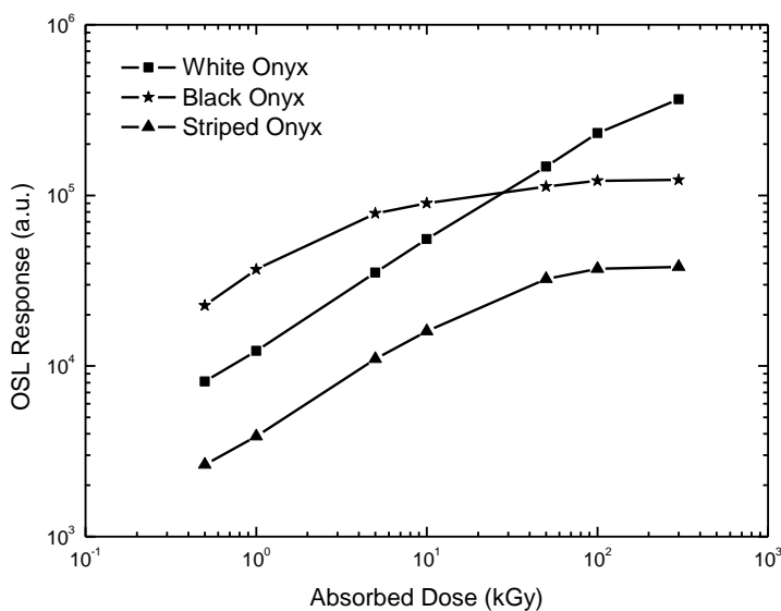
Figure 2. Dose-OSL response curves of Onyx-Teflon pellets for 60 Co radiation
