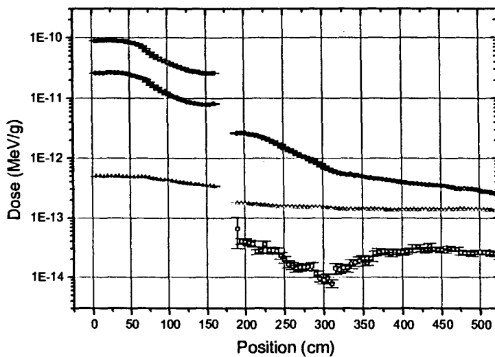
Figure 4. Dose distribution profiles obtained by MCNP simulations along a single axis in a cylindrical symmetrical configuration. Black squares correspond to neutron dose; red circles: secondary gammas (n,g); green triangles: sample gammas.
