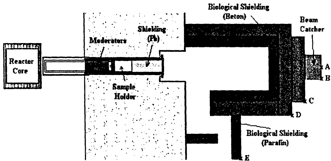
Figure 1. Schematic view of the BNCT facility which is under construction in BH#3 of IEA-R1 Reactor in IPEN.
