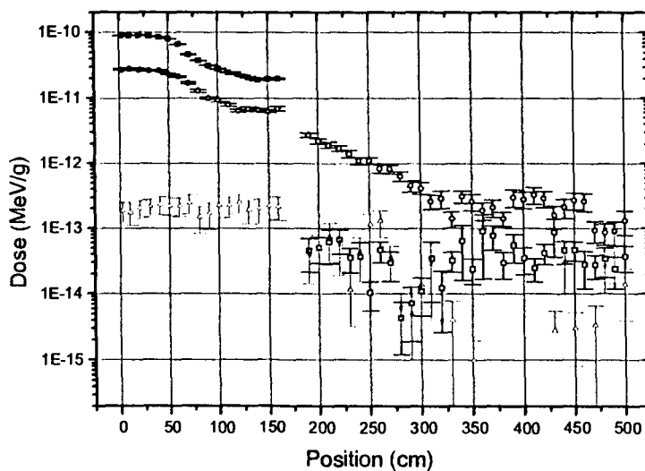
Figure 5. Dose distribution profiles obtained by MCNP simulations along a single axis in a real modeled configuration. Black squares correspond to neutron dose; red circles: secondary gammas (n,g); green triangles: sample gammas.
