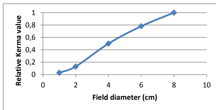
Figure 3. Simulated KAP meter behavior varying the field diameter.
