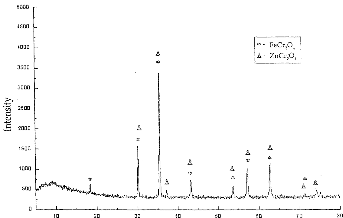
Figure 1. X-ray diffractogram of pigment obtained with 20% of the waste.
