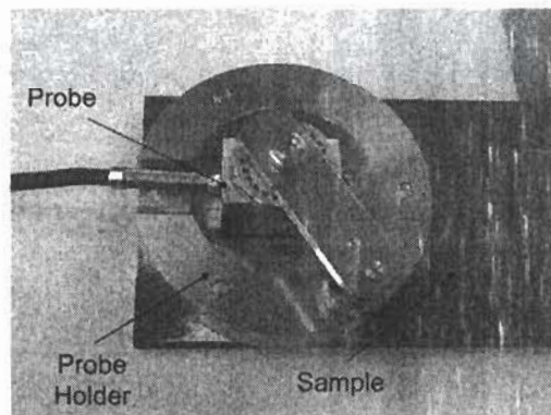
Figure 2. Experimental set-up used to verify the angular dependence of the MBN.
