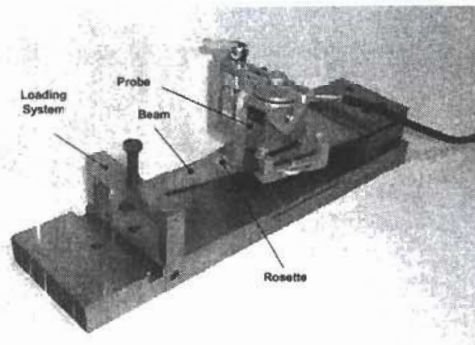
Figure 1. Experimental set-up used to obtain tension stresses (a) and compression stresses (b) at the beams surface.
