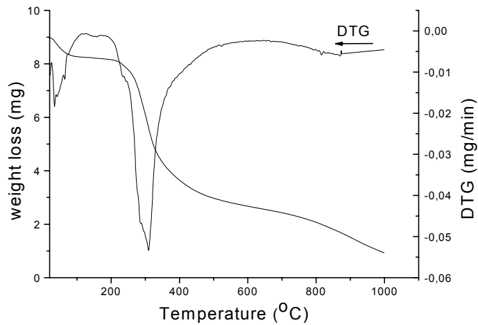
Fig.2 – TGA/DTG curves of albumin, heated rate 5^\circ\text{C}/\text{min} in sintetic air.
