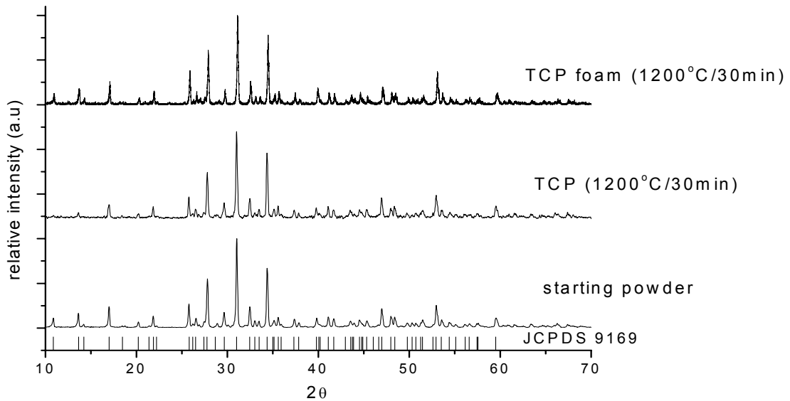
Fig. 3 - X-ray diffraction patterns for samples in different conditions (starting powder, TCP, sintered at 1200°C/30min and TCP foam based albumin sintered at 1200°C/30min).
