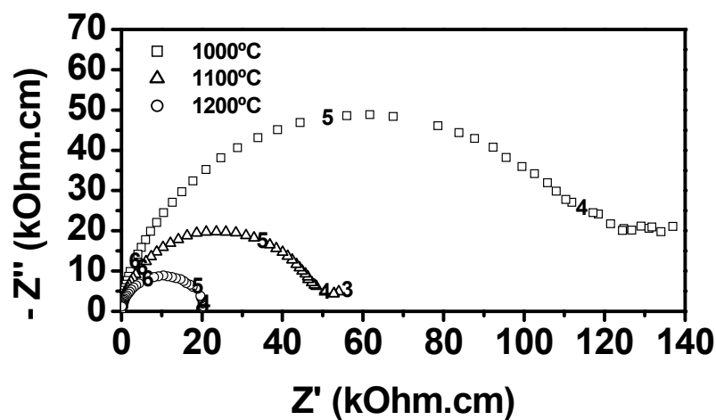
Fig. 4. Impedance diagrams of La \beta -Al _2 O _3 sintered at 1600 °C/ 2 h measured at different temperatures. The numbers stand for the logarithm of the frequency (Hz).
