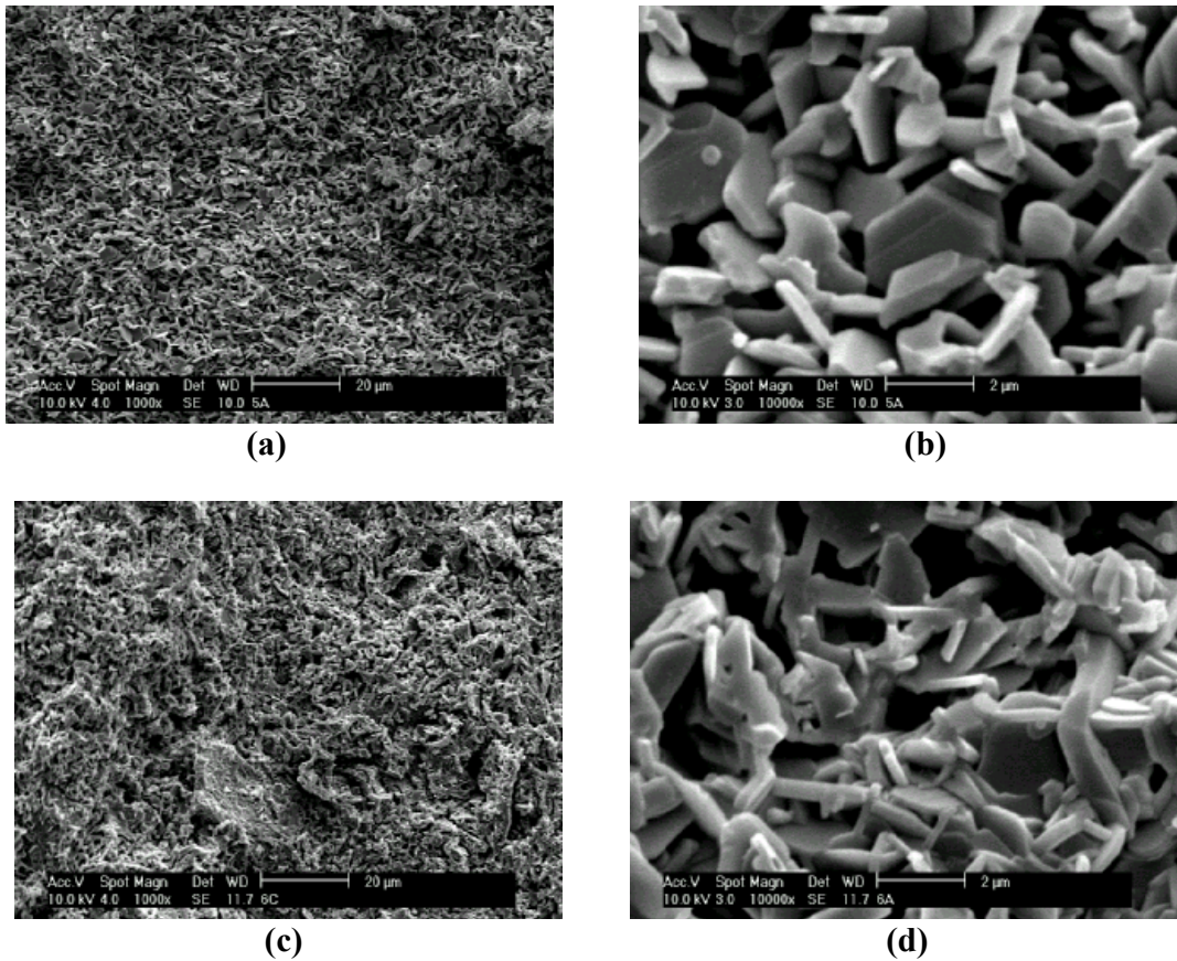
Fig. 3. Scanning electron microscopy micrographs of La \beta -Al _2 O _3 pellets sintered at 1600 °C/2 h: before attrition (a) magnification 1000X and (b) magnification 10000X; after attrition (c) magnification 1000X and (d) magnification 10000X.
