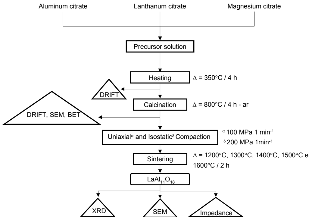
Fig. 1. Flowchart of the experimental procedure to obtain La \beta -Al 2 O 3 by the polymeric precursor method.
