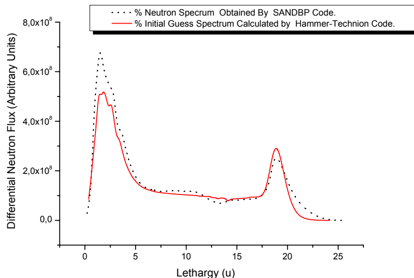
Figure 3. Comparative Graphics between Initial Guess Spectrum calculated by Hammer-Technion Cellular Code and that obtained by Experimental Values Using the SANDBP Code. The Spectrum is presented in Lethargy Units.
