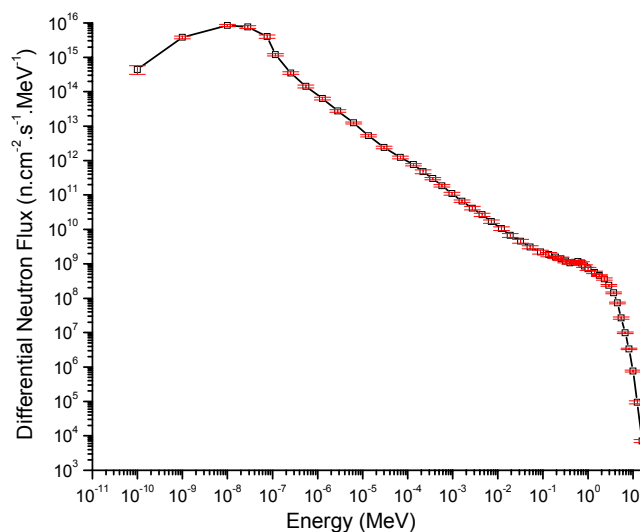
Figura 2. Neutron Spectrum at the Central Position of the IPEN/MB-01 Reactor Core obtained by SANDBP Code (3 iterations) to 51 energy points /5/.
