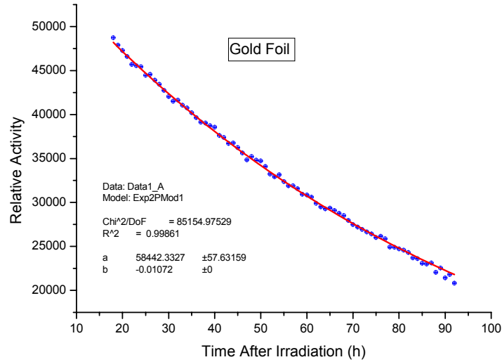
Figure 1 – Decay Curve to Au Foil.
