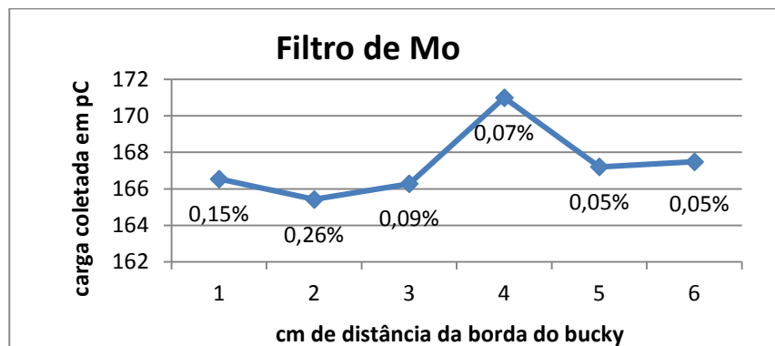
Figure 4: Graphic of measurements made using Mo filter. The vertical column indicates the reading Load pC, and the horizontal region in cm where the ionization chamber was placed. Demonstrates that the region where there was the highest reading load was 4 cm.
