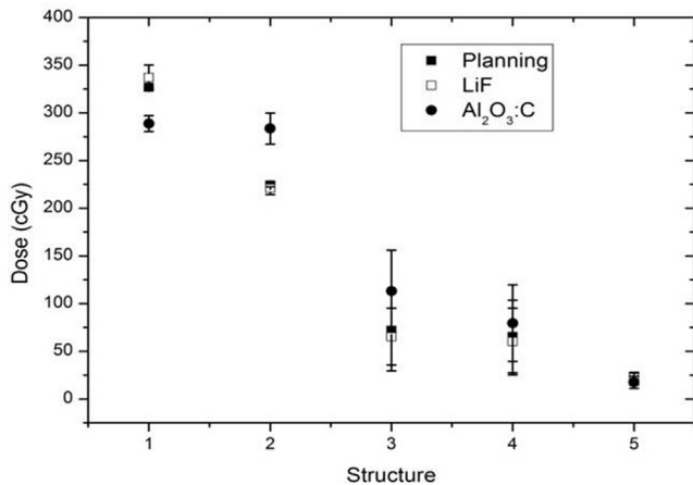
Fig. 4. Mean doses given by the planning system and measured by LiF:Mg,Ti and Al 2 O 3 :C.
