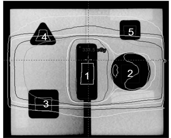
Fig. 3. Isodose curves given by planning system showing the dose distribution in the five phantom cavities.
