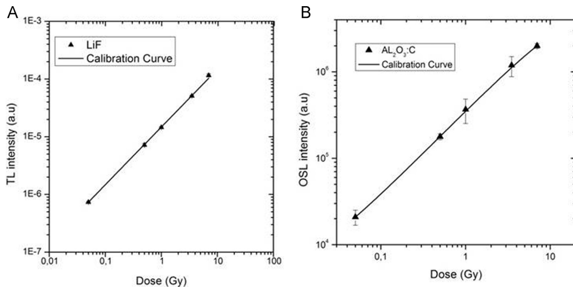
Fig. 2. Dose–response curves to 6 MV photon beam from linear accelerator VARIAN 6EX of (A) LiF:Mg using TL technique, Ti and (B) \text{Al}_2\text{O}_3\text{:C} using OSL technique.
