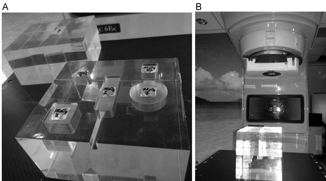
Fig. 1. (A) PMMA phantom containing five cavities and PMMA block and (B) dosimeters positioned inside the phantom's cavities and PMMA block positioned on top of the phantom to ensure backscattering.
