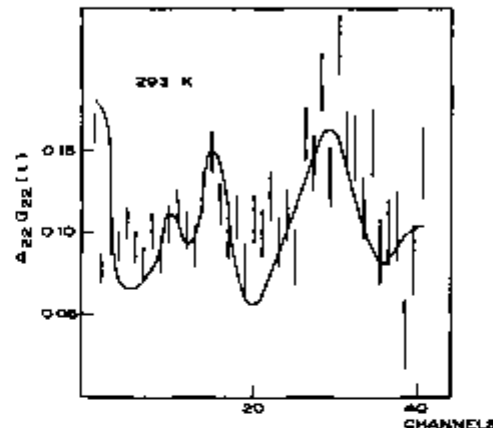
Figure 2 - A_{22}G_{22}(t) Coefficient at the ^{111}\text{Cd} Site In \text{CdTiO}_3 for the Neutron Activated Sample Calibration: 5 nsec/channel
