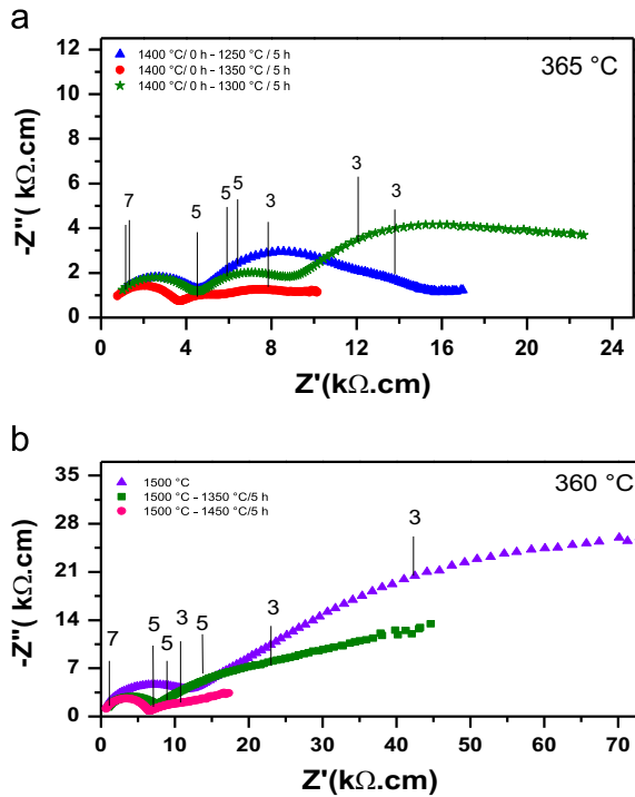
Fig. 5. Impedance spectroscopy diagrams of LSGM sintered at (a) 1400 °C and (b) 1500 °C ( T_1 ) and several T_2 ( t_2=5 h).
