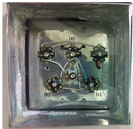
Figure 1. Top view of the LED-based irradiator. Red LEDs were placed on (a), (b) and (c).
