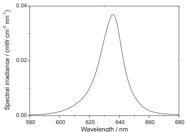
Figure 2. Spectral irradiance of the red LED-based irradiator.
