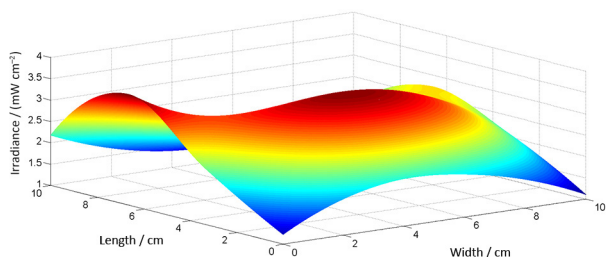
Figure 3. Irradiance distribution of the LED-based irradiator.
