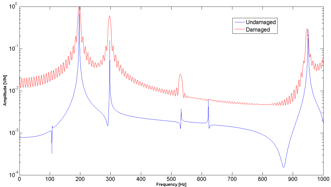
Figure 6: FRF using piezoelectric transducer: cylinder intact vs. damaged cylinder
