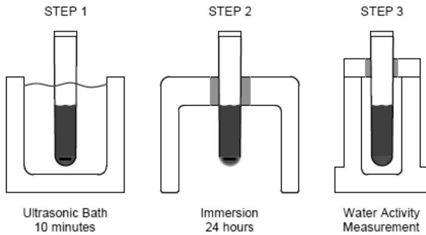
Fig. 2 The three steps of the leakage immersion test.
