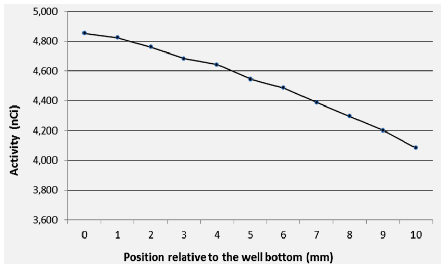
Fig. 4 Measured activity with variable vertical positioning in the well detector.
