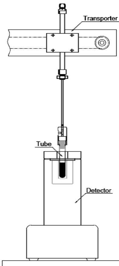
Fig. 5 Automated device to perform the sample positioning in the detector.
