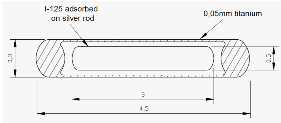
Fig. 1 Iodine-125 seed developed at IPEN.
