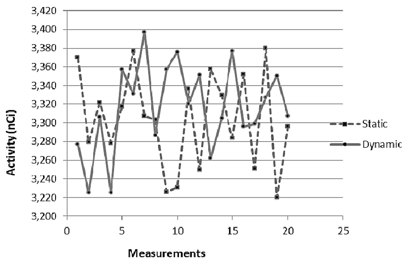
Fig. 6 Results obtained for both “static” and “dynamic” assays.
