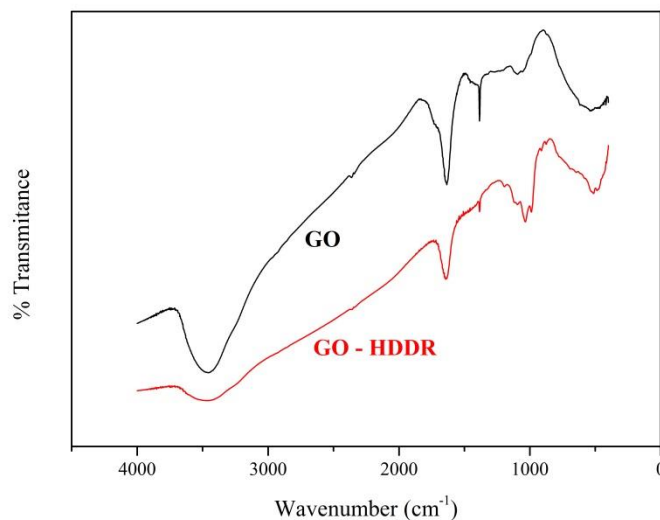
Figure 7. FTIR spectra of GO (black) and GO after HDDR process (red).
