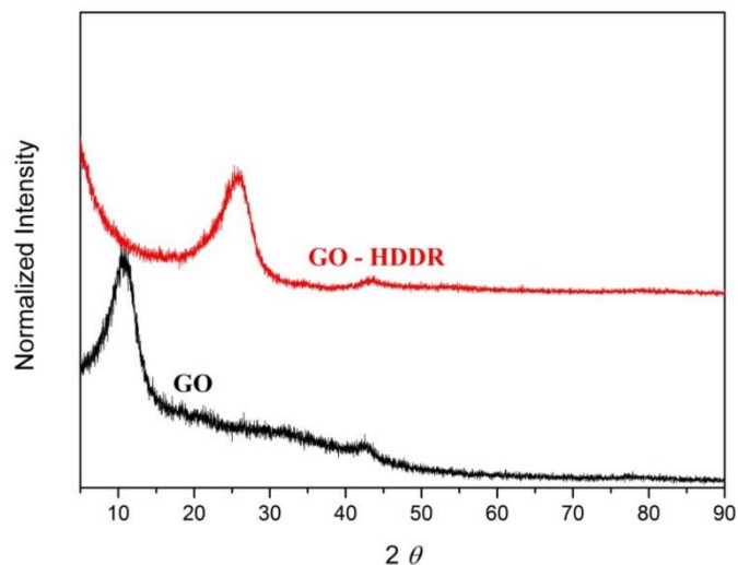
Figure 5. XRD of the GO starting material and after treatment using the standard HDDR process.
