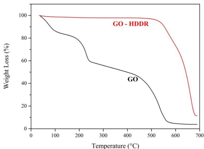
Figure 6. TGA plots of GO (black) and GO after HDDR process (red).
