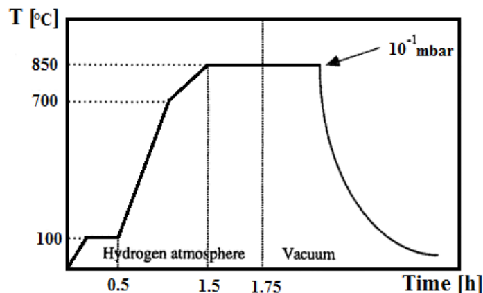
Figure 3. Schematic diagram of the HDDR treatment cycle [9].
