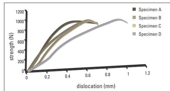
FIGURE 4 - Strength x Dislocation graph presenting the flexure test curves for the four specimens tested.
