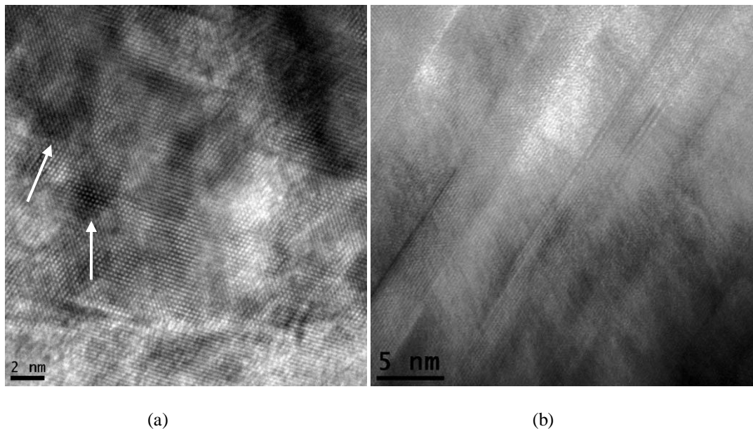
Figure 9: Electron micrograph of the sample of Ti-6Al-4V, after heat treatment 1000 ° C/1h and rapid cooling in water.
