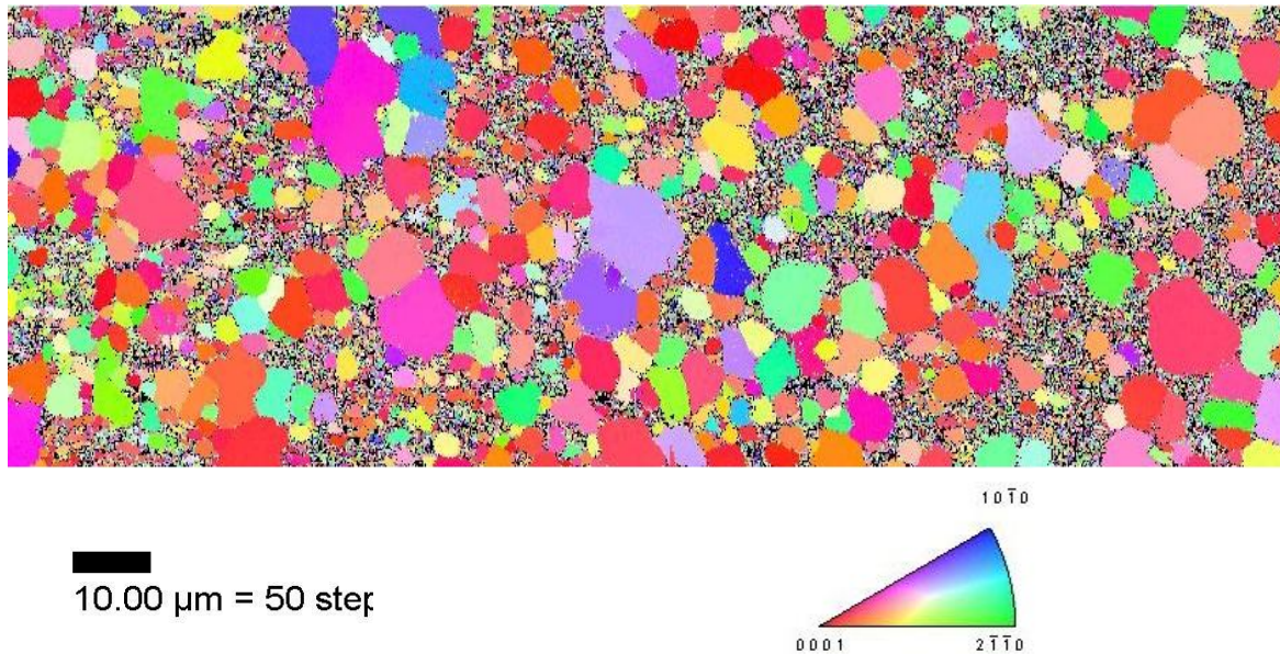
Figure 6: SEM/EBSD image of Ti-6Al-4V microstructure annealed at 800°C for two hours.
