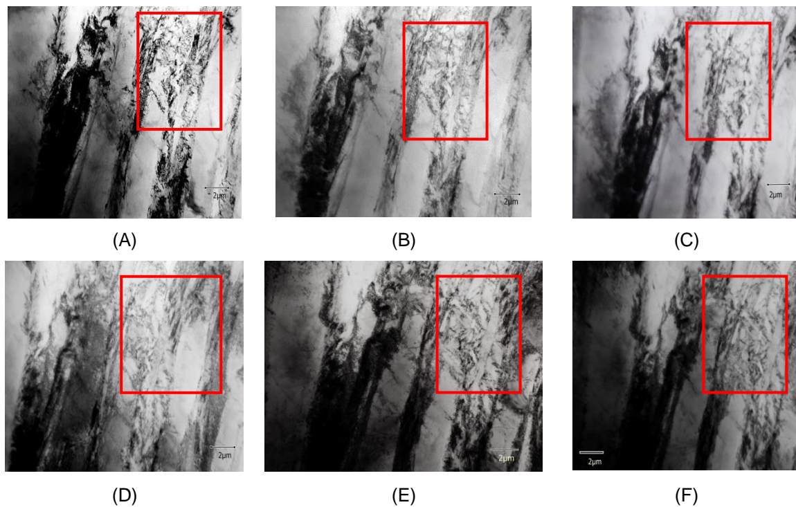
Figure 3: Electronic micrographs of Ti-6Al-4V sample on the analysis of in situ traction for different shifts: (A) 0.05mm, (B) 0.10 mm, (C) 0.15 mm, (D) 0.20 mm, (E) and (F) 0.25 mm.
