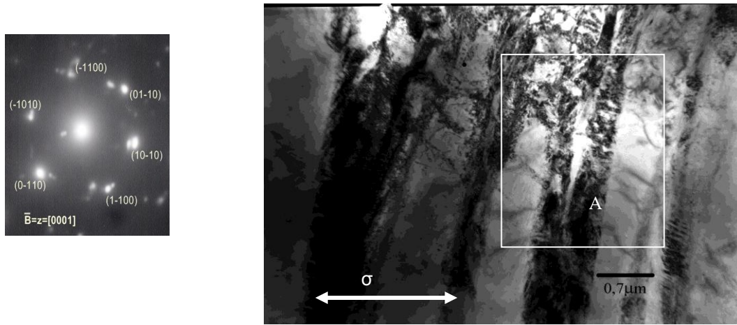
Figure 2: Electron micrograph of the sample of Ti-6Al-4V and its diffraction pattern from the region indicated in A
