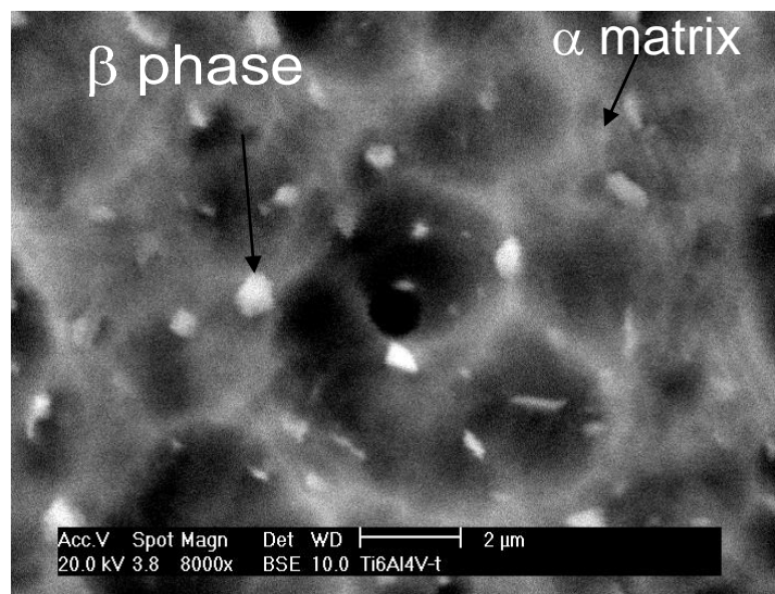
Figure 5: SEM image of microstructure of the sample Ti-6Al-4V annealed at 800°C for two hours
