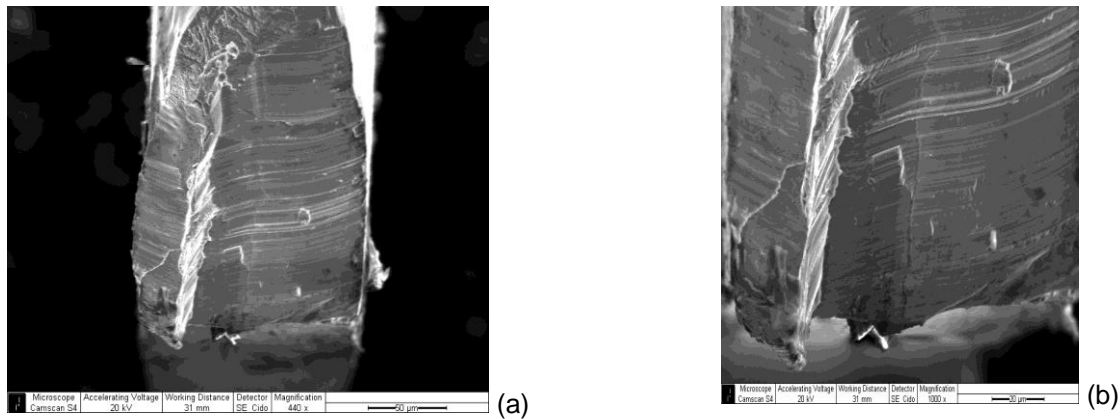
Figure 7: SEM micrograph of Ti-6Al-4V, after heat treatment at 1000 °C/1h and rapid cooling in water at two different magnifications
