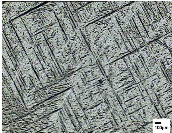
Figure 4. Optical micrograph of the sample of Ti-6Al-4V heat treated at 1000 °C for two hours and cooled in water submitted to surface chemical attack
