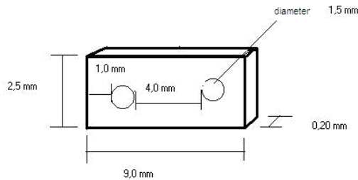
Figure 1: Scheme of specimen for in situ TEM tensile test
