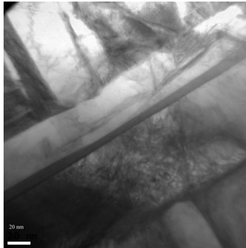
Figure 8: Electron micrograph of the sample of Ti-6Al-4V, after heat treatment 1000 ° C/1h and rapid cooling in water.
