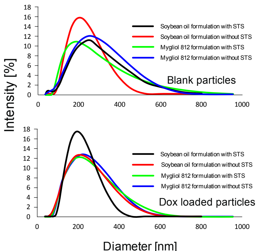
Figure 1. Freshly prepared carrier systems display a peak hydrodynamic particle size of approximately 200 nm. Freshly prepared particles (blank: top panel; doxorubicin (Dox)-loaded particles: bottom panel) were diluted 1:2500 in particle-free water and measured using a Malvern particle size reader. The distribution of the hydrodynamic particle size (in nm) is plotted against the intensity (in %). Individual preparations are denoted by black: soybean oil formulation with sodium tetradecyl sulfate (STS); red: soybean oil formulation without STS; green: Mygliol 812 formulations with STS; blue: Mygliol 812 formulations without STS.
