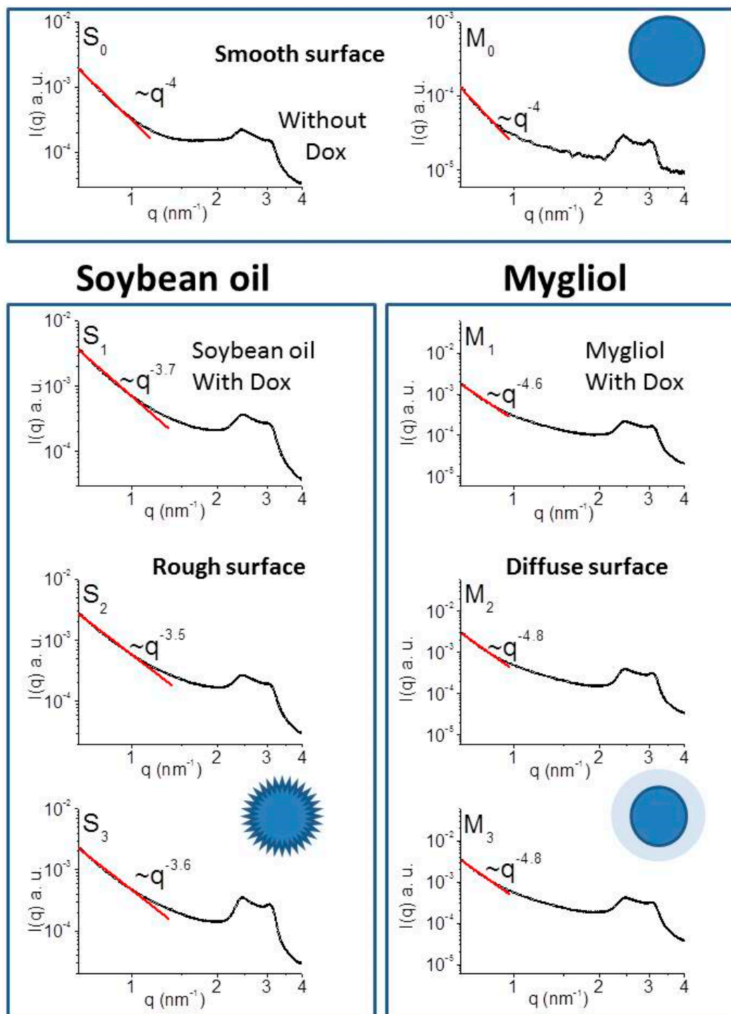
Figure 6. Loading with Dox abrades the surfaces of STS-containing soybean oil carriers. Shown here are the results of SAXS measurements using STS-containing Mygliol 812 (M) and Soybean (S) oil-based carriers with S 0 and M 0 denoting plain formulations, and Dox-loaded carriers labeled with the amounts of Dox loaded (M 1 : 180 \mu M; S 1 : 360 \mu M; M 2 and S 2 : 540 \mu M; M 3 and S 3 : 900 \mu M). The intensity of the scattering event I is plotted using arbitrary units against the scattering vector q in nm -1 with the approximated tangent of the graph denoted as red line in the respective plots. In addition, a graphical interpretation of the results obtained is provided. Both plain soybean oil and plain Mygliol 812-based systems display a smooth surface in accordance with [30]. Loading with Dox, regardless of the amounts loaded, roughens the surface in the case of soybean oil carriers. In stark contrast, Mygliol 812-based formulations yield a diffuse surface after loading with Dox.
