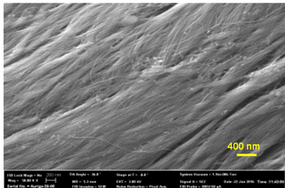
Figure 5. SEM images of CNT yarn gamma irradiated at 100 kGy.
