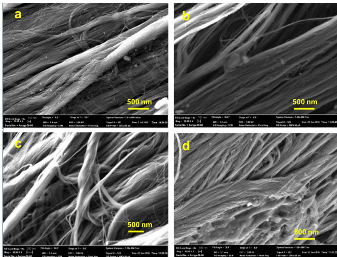
Figure 4. SEM images of CNT yarn e-beam irradiated at 800 kGy.
