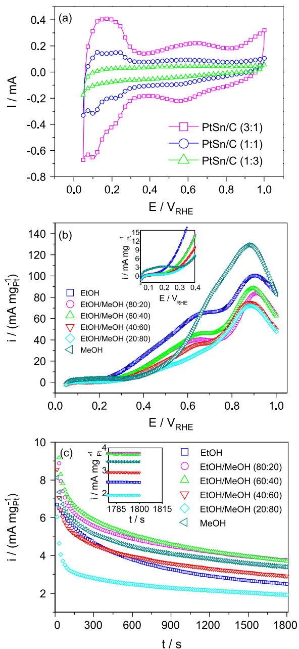
Figure 2. (a) Cyclic voltammograms ( v = 0.05 \text{ V s}^{-1} ) in H_2SO_4 (0.5 mol L -1 ) of the PtSn/C (3:1), PtSn/C (1:1) and PtSn/C (1:3) electrocatalysts prepared by polymeric precursor method; (b) cyclic voltammograms ( v = 0.01 \text{ V s}^{-1} ) and (c) chronoamperometries obtained from the oxidation of solutions (1 mol L -1 ) containing MeOH and EtOH in different volume ratios using PtSn/C (3:1) in H_2SO_4 (0.5 mol L -1 ), with E = 0.5 \text{ V} for 1800 s. T = 25 \text{ }^\circ\text{C} .
