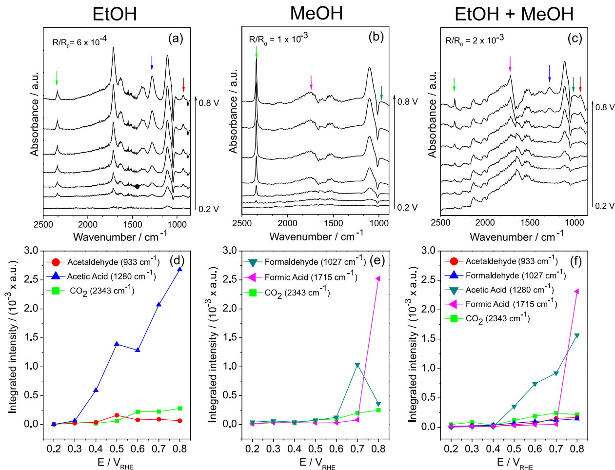
Figure 3. In situ ATR-FTIR spectra of the products and their corresponding integrated intensities obtained for the oxidation of (a) and (d) ethanol (EtOH, 1 mol L -1 ); (b) and (e) methanol (MeOH, 1 mol L -1 ); (c) and (f) mixtures of ethanol and methanol in a volume ratio of 80:20 (1 mol L -1 ) using the Pt 3 Sn 1 /C electrocatalyst in HClO 4 (0.1 mol L -1 ) media.
