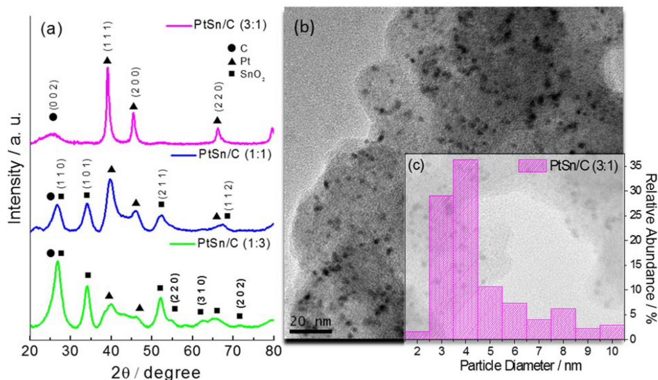
Figure 1. (a) X-ray diffractograms of the PtSn/C (3:1), PtSn/C (1:1) and PtSn/C (1:3) electrocatalysts prepared using the polymeric precursor method. Transmission electron microscopy (b) image and (c) size distribution histogram for the PtSn/C (3:1) electrocatalyst.
