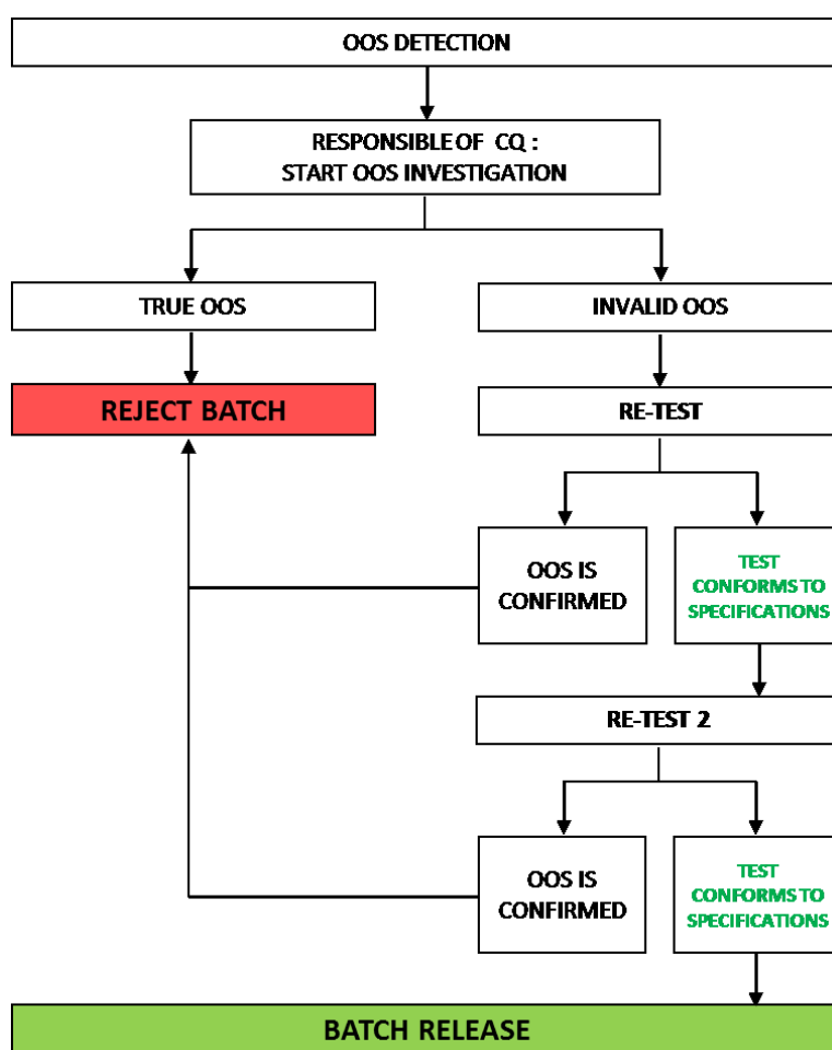
FIG. 4. Decision Tree
