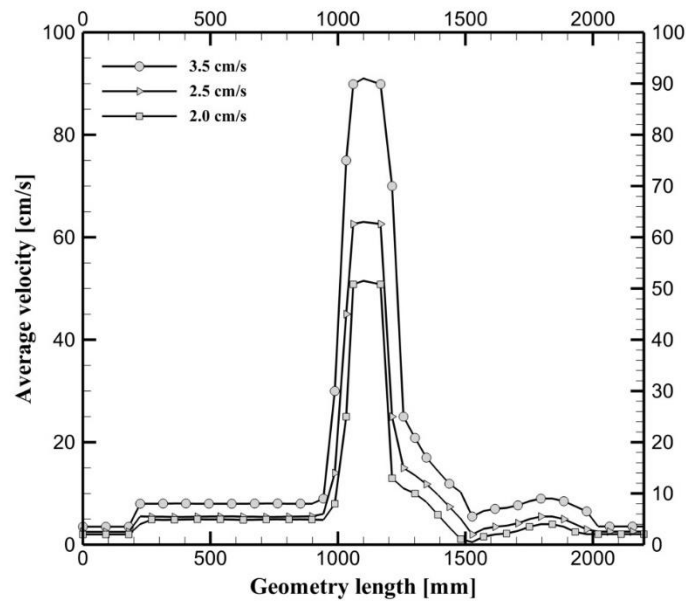
Figure 6: Average velocity for long blockage
