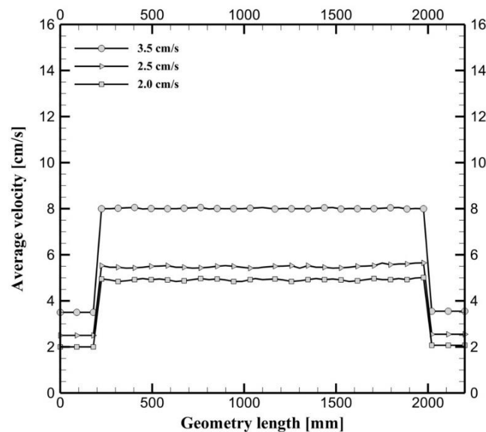
Figure 5: Average velocity for zero blockage
