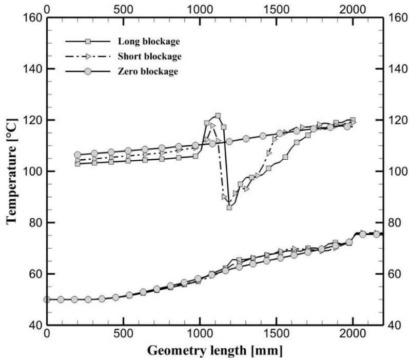
Figure 10: Thermal behavior for solid/fluid with 3,5 cm/s
