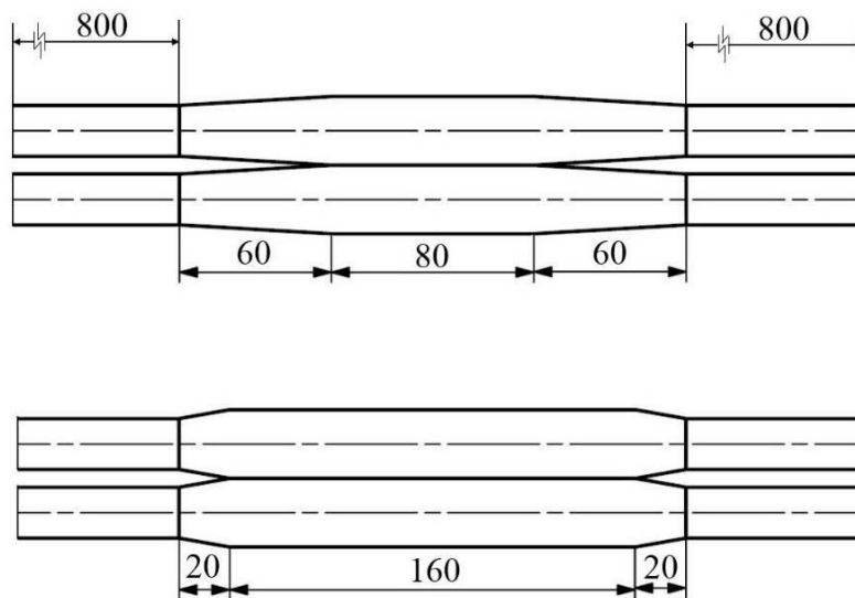
Figure 2: Short and long blockage geometries
