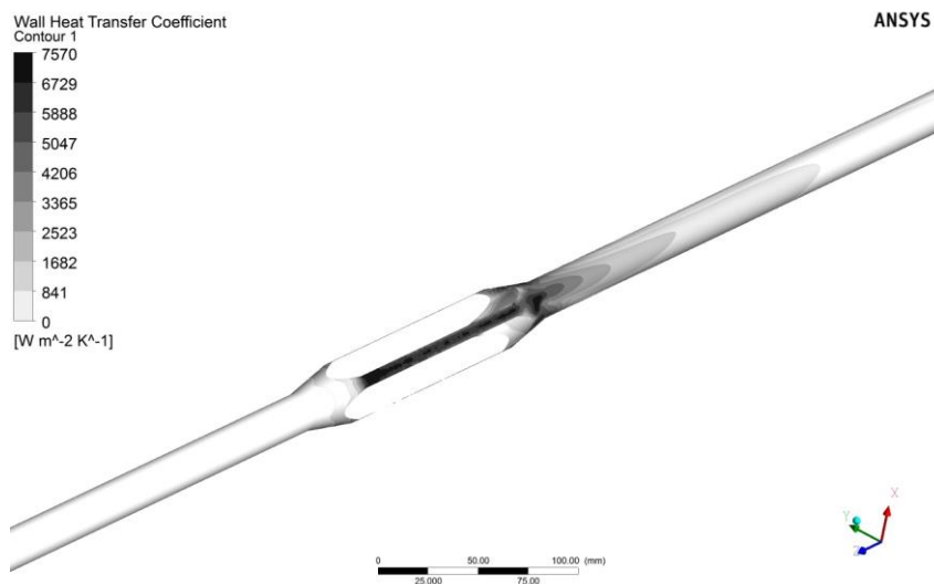
Figure 12: Wall heat transfer coefficient for long blockage (3.5cm/s)
