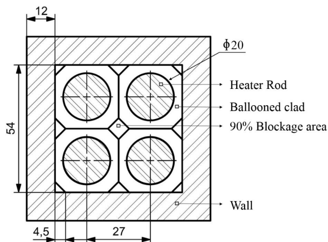
Figure 1: Top view of fuel rods
