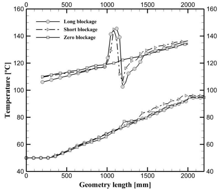
Figure 8: Thermal behavior for solid/fluid with 2cm/s
