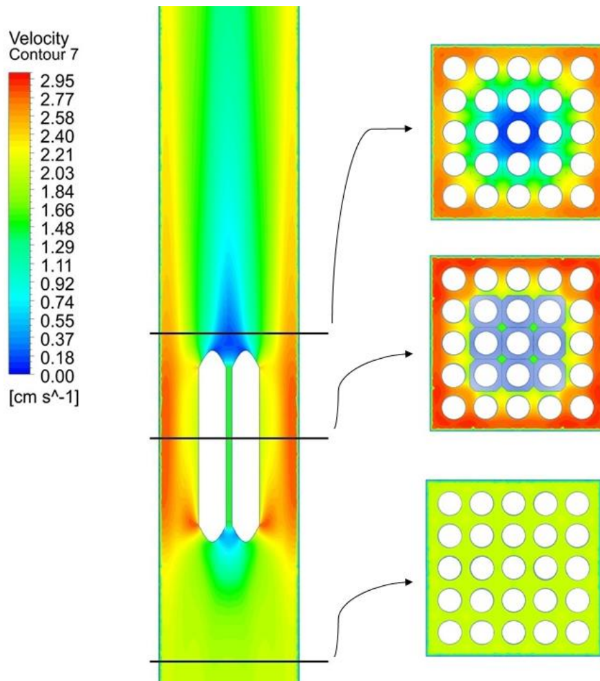
Figure 13: 5x5 assembly with colored map for velocity
