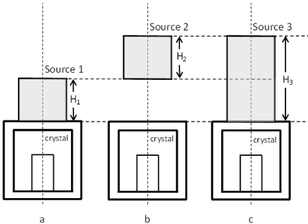
Fig. 1. Measurement configurations.
