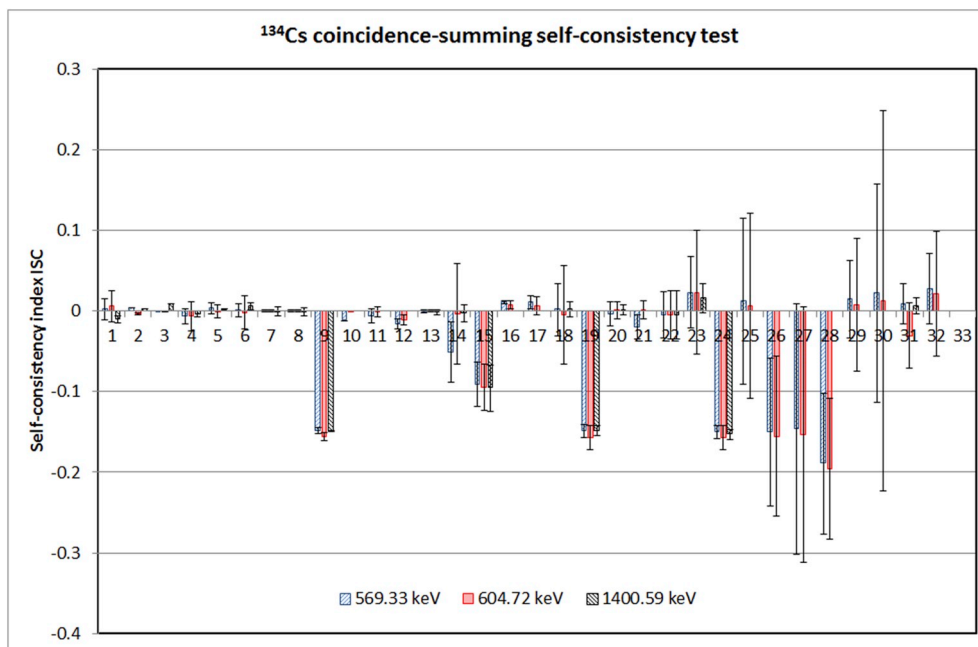
Fig. 4. Self-consistency index for several peaks of ^{134}\text{Cs} . The values of ISC(NP) for the 569.33 keV and 604.72 keV peaks, and of ISC(SP) for the 1400.59 keV peak are displayed in function of the code of the participants.
