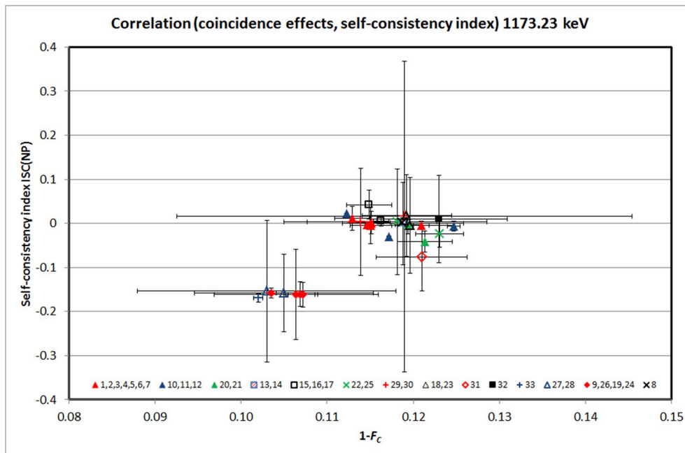
Fig. 6. The distribution of the self-coincidence index as a function of the magnitude C of coincidence summing effects in configuration (a) for the 1173.23 keV peak of 60 Co.
