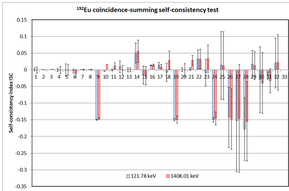
Fig. 5. Self-consistency index for 152 Eu peaks of energy 121.78 keV and 1408.01 keV. The values of ISC(NP) are displayed in function of the code of the participants.
