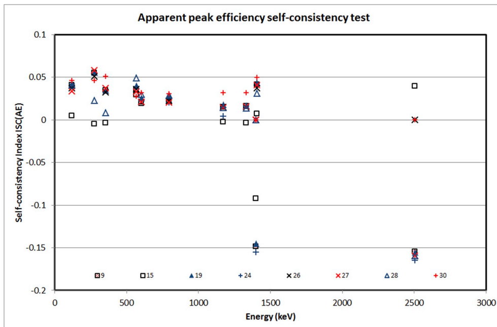
Fig. 9. The self-consistency index for the apparent peak efficiency for the sets of results in which at least one absolute value of \text{ISC}(\text{AE}) > 0.05 . The uncertainty bars were removed for avoiding a too clumsy figure.
