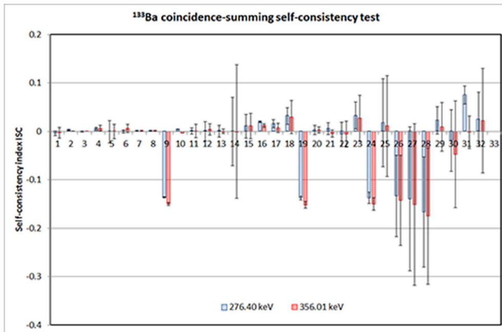
Fig. 3. Self-consistency index for ^{133}\text{Ba} peaks of energy 276.40 keV and 356.01 keV. The values of ISC(NP) are displayed in function of the code of the participants.
