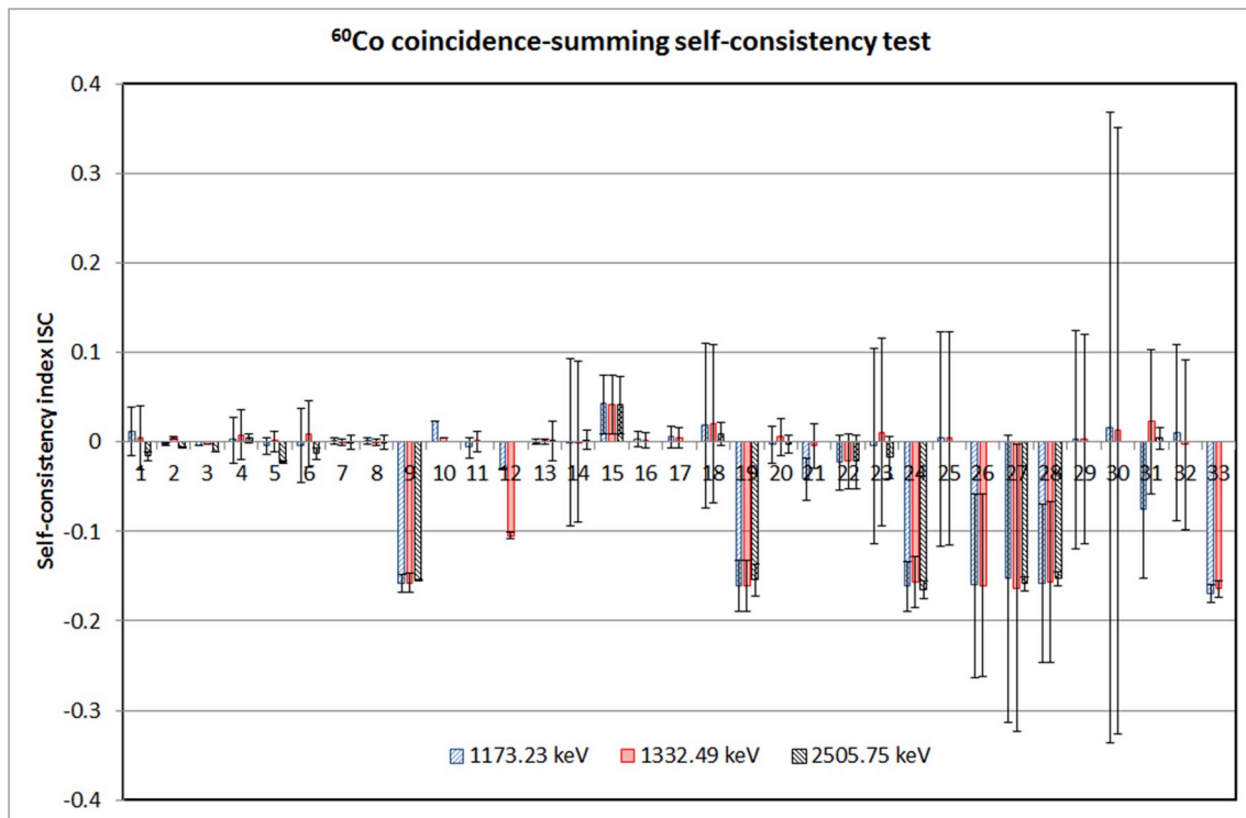
Fig. 2. Self-consistency index for ^{60}\text{Co} peaks. The values of ISC(NP) for the 1173.23 keV and 1332.49 keV peaks, and of ISC(SP) for the 2505.75 keV peak are displayed in function of the code of the participants. The uncertainty bars correspond to 1\sigma .
