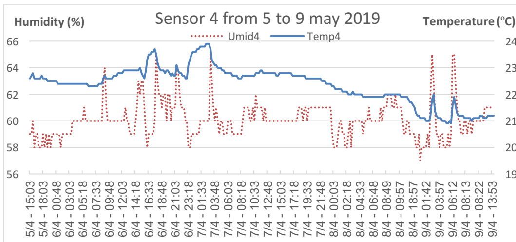
Figure 4 - Temperature (Temp) and humidity (Umid) in S4 for the period from 5-9 may/2019.
