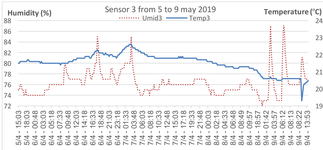
Figure 6 - Temperature (Temp) and humidity (Umid) in S3 for the period from 5-9 may/2019.
