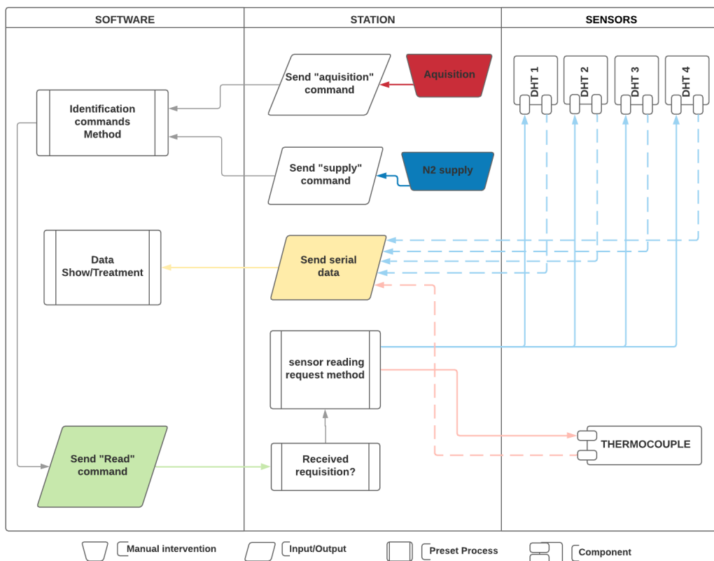
Figure 2 - Workflow between software, station and sensors
