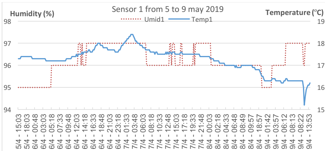
Figure 7 - Temperature (Temp) and humidity (Umid) in S1 for the period from 5-9 may/2019.
