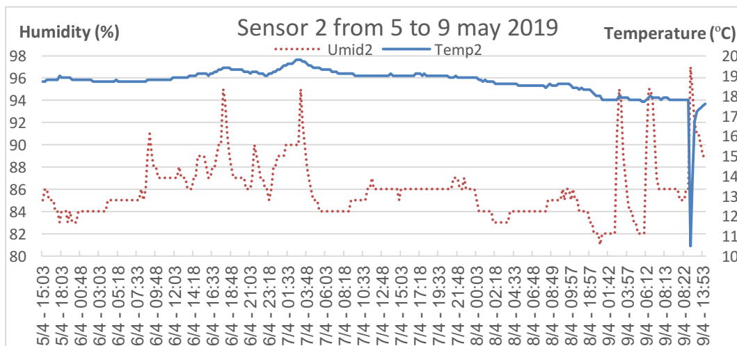
Figure 5 - Temperature (Temp) and humidity (Umid) in S2 for the period from 5-9 may/2019.
