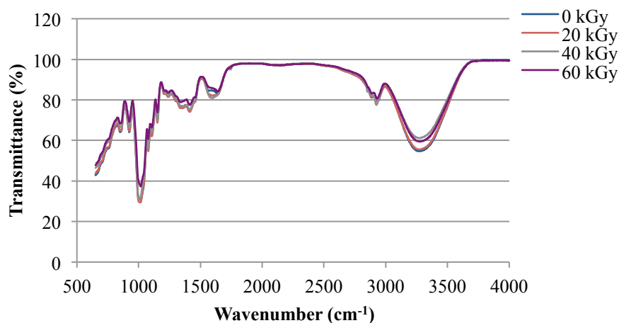
Figure 1: FTIR spectra of starch film containing hibiscus aqueous extract.
