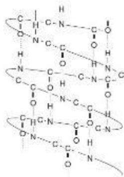
Figure 2: Keratin structure [4]
