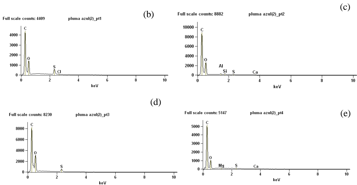
Figure 8: EDS analysis for 4 selected points for Feather 5. Accelerating Voltage: 8.0 kV Magnification: 500. Detector: UltraDry (a, b, c, d, e)
