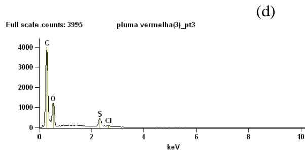
Figure 9: EDS analysis for 4 selected points for Feather 31. Accelerating Voltage: 8.0 kV. Magnification: 500. Detector: UltraDry (a, b, c, d, e)
