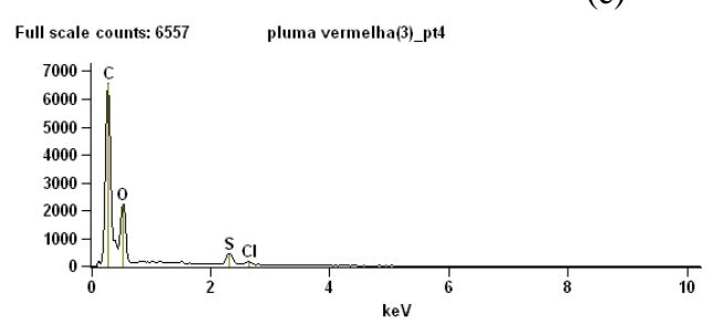
Figure 9: EDS analysis for 4 selected points for Feather 31. Accelerating Voltage: 8.0 kV. Magnification: 500. Detector: UltraDry (a, b, c, d, e)
