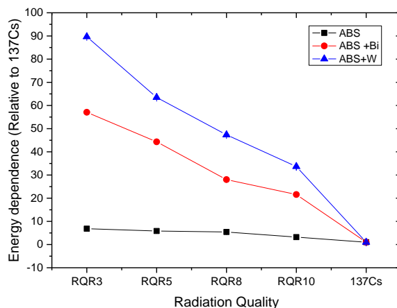
Figure 7. Energy dependence of the printing materials
