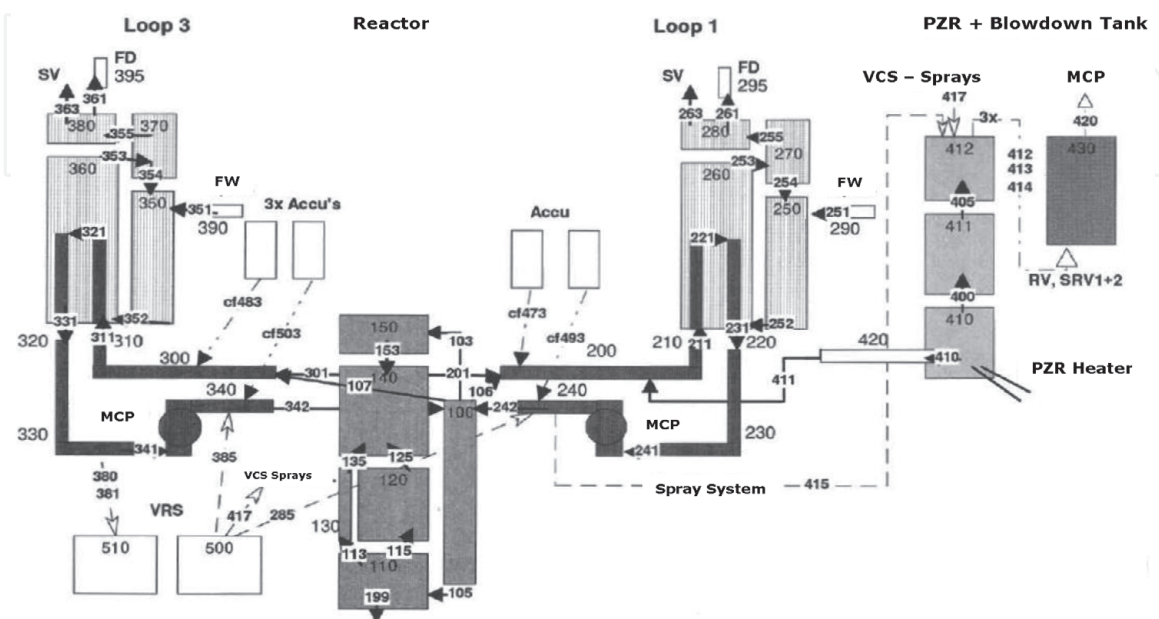
Figure 1. PWR primary and secondary circuit modeling.
