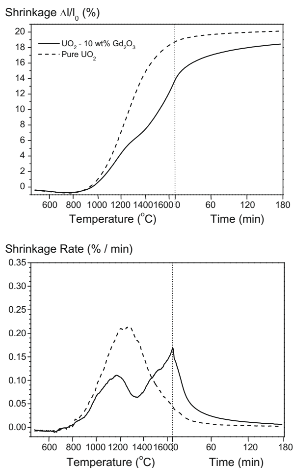
Fig. 1. Effect of Gd_2O_3 on the sintering behavior of UO_2-Gd_2O_3 fuel pellets (dry mechanical blending/5 °C/min).
