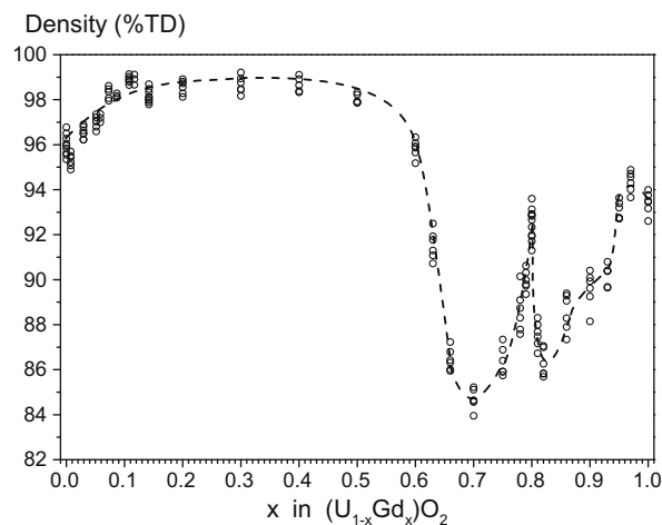
Fig. 2. Effect of the gadolinium concentration on the sintered density of (U,Gd)O_2 pellets prepared by coprecipitation (solid solution).
