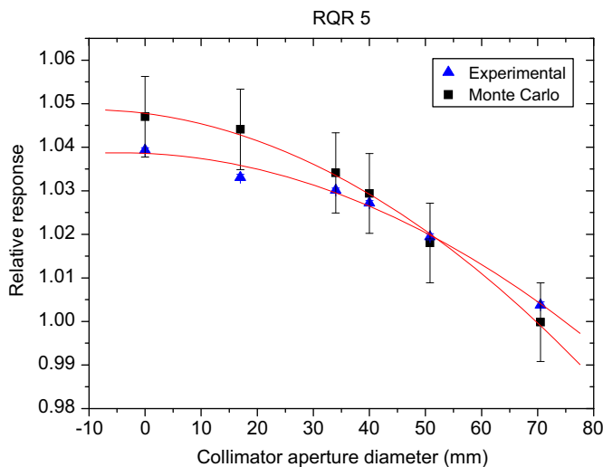
Fig. 4. Backscattered X-radiation effect in the transmission ionization chamber response for diagnostic radiology level RQR 5, for experimental measurements and Monte Carlo technique.
