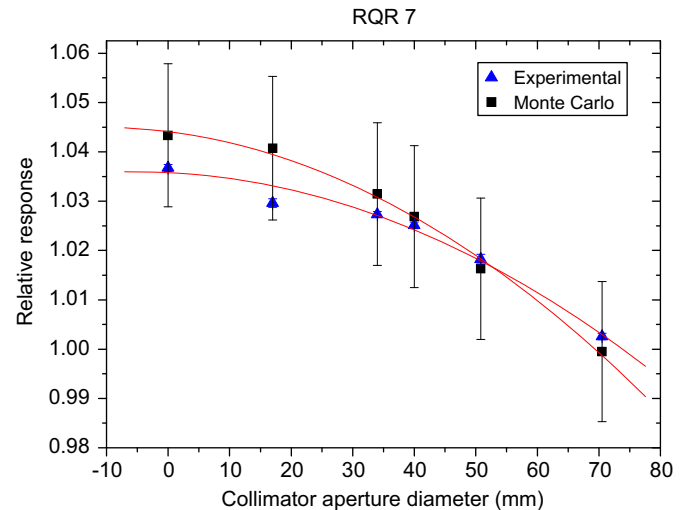
Fig. 5. Backscattered X-radiation effect in the transmission ionization chamber response for diagnostic radiology level RQR 7, for experimental measurements and Monte Carlo technique.
