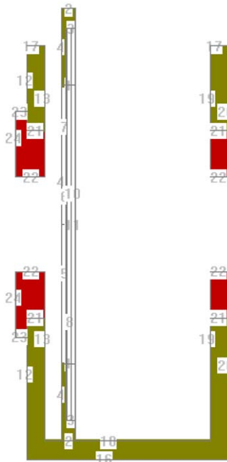
Fig. 2. Geometry of the transmission ionization chamber and the collimation system as implemented in the MCNP inputs.
