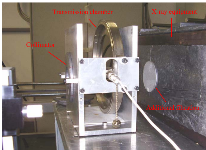
Fig. 1. Transmission ionization chamber and collimation system positioned in front of an X-ray equipment at the Calibration Laboratory of IPEN.
