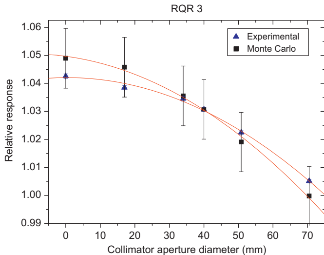
Fig. 3. Backscattered X-radiation effect in the transmission ionization chamber response for diagnostic radiology level RQR 3, for experimental measurements and Monte Carlo technique.
