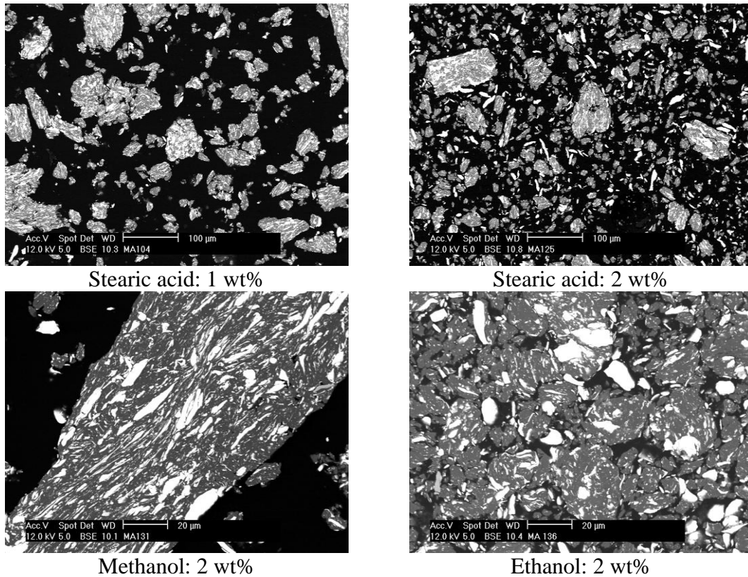
Fig. 2 – Microstructure of aggregates produced after milling with different PCAs.
