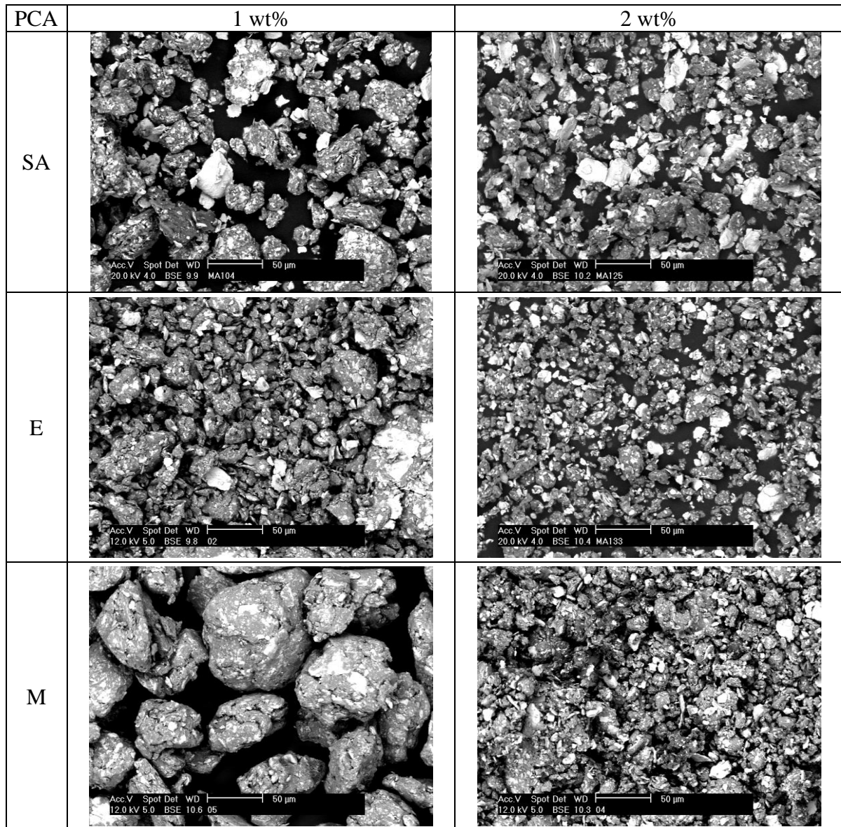
Fig. 1 – SEM images (backscattered electrons) of as-milled powders with different types and amounts of PCAs (SA = Stearic Acid; E = Ethanol; M = Methanol).
