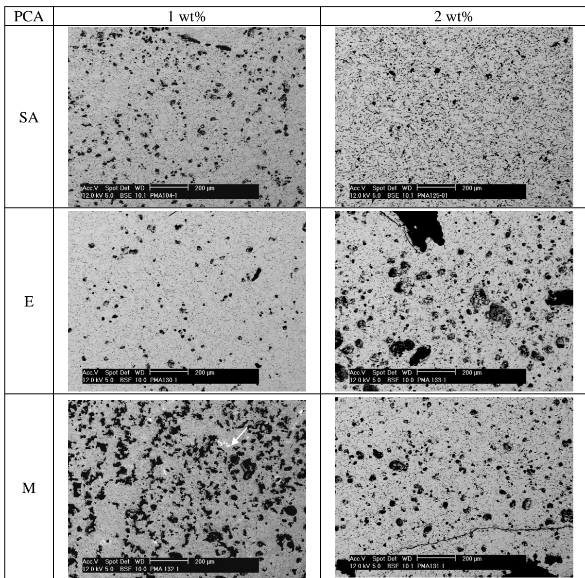
Fig. 4 – Microstructure of reacted pellets for different PCAs additions.
