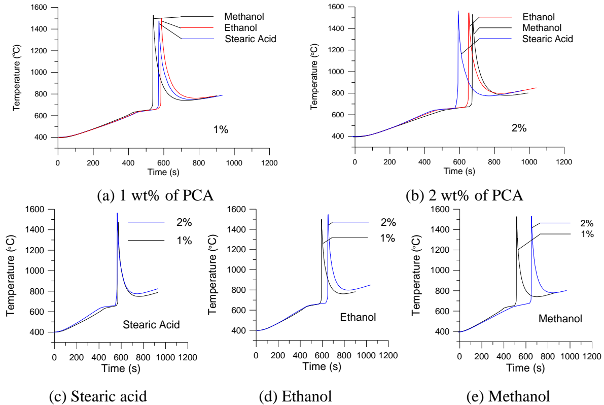
Fig. 4 – Temperature profiles of pellets grouped by content (a, b) and type of PCA (c, d, e).
