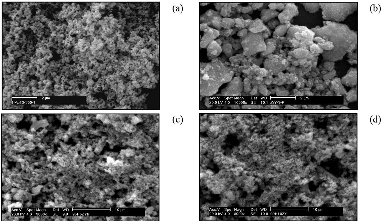
Fig. 1: SEM micrographs of powders: (a) H; (b) 3YSZ, (c) 95H5ZY and (d) 90H10ZY.
