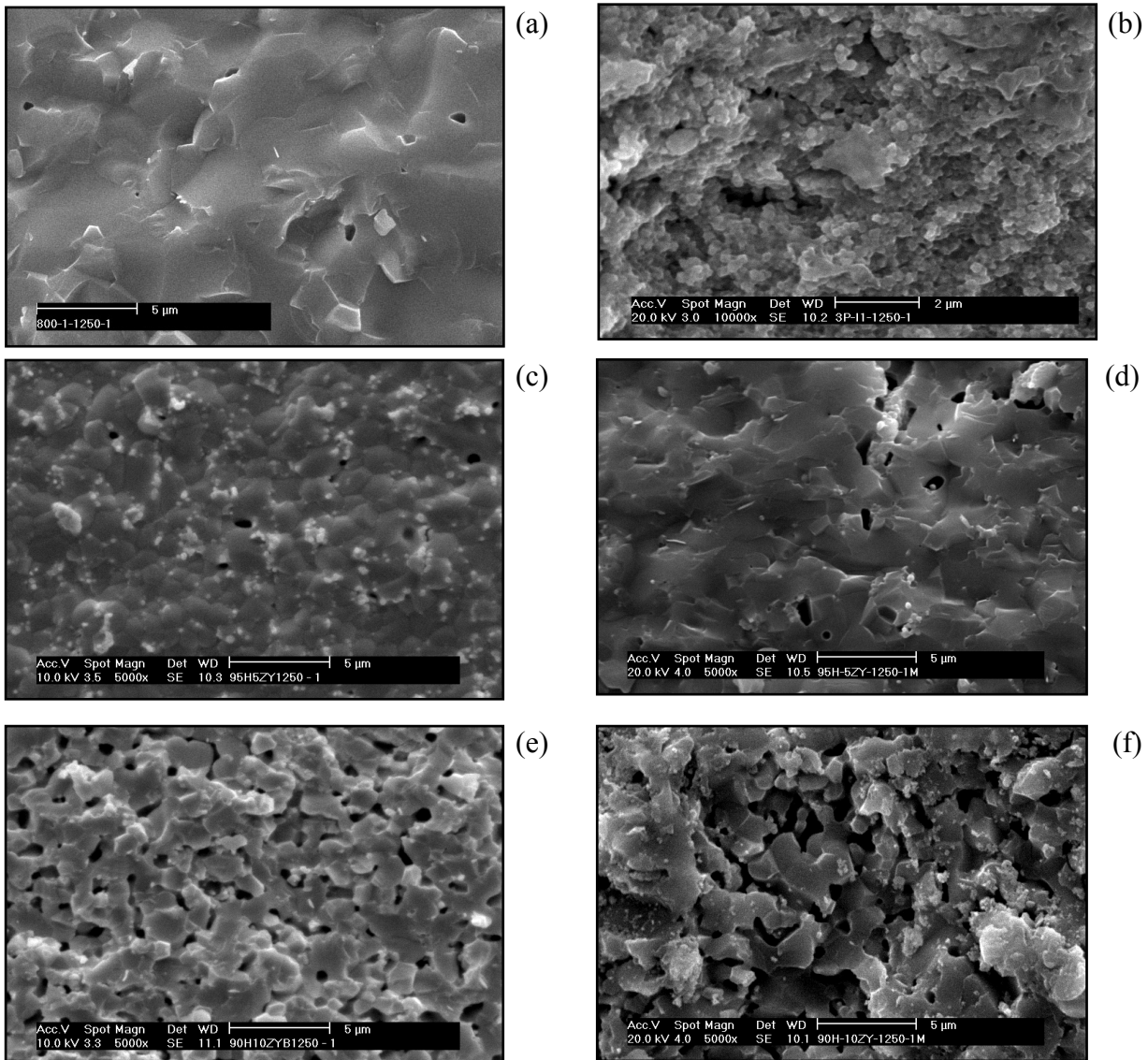
Fig. 2: SEM micrographs of ceramic samples sintered at 1250°C for 1 hour: (a) H; (b) 3YSZ, (c) 95H5ZY, (d) 95H5ZY – M, (e) 90H 10ZY and (f) 90H 10ZY – M.
