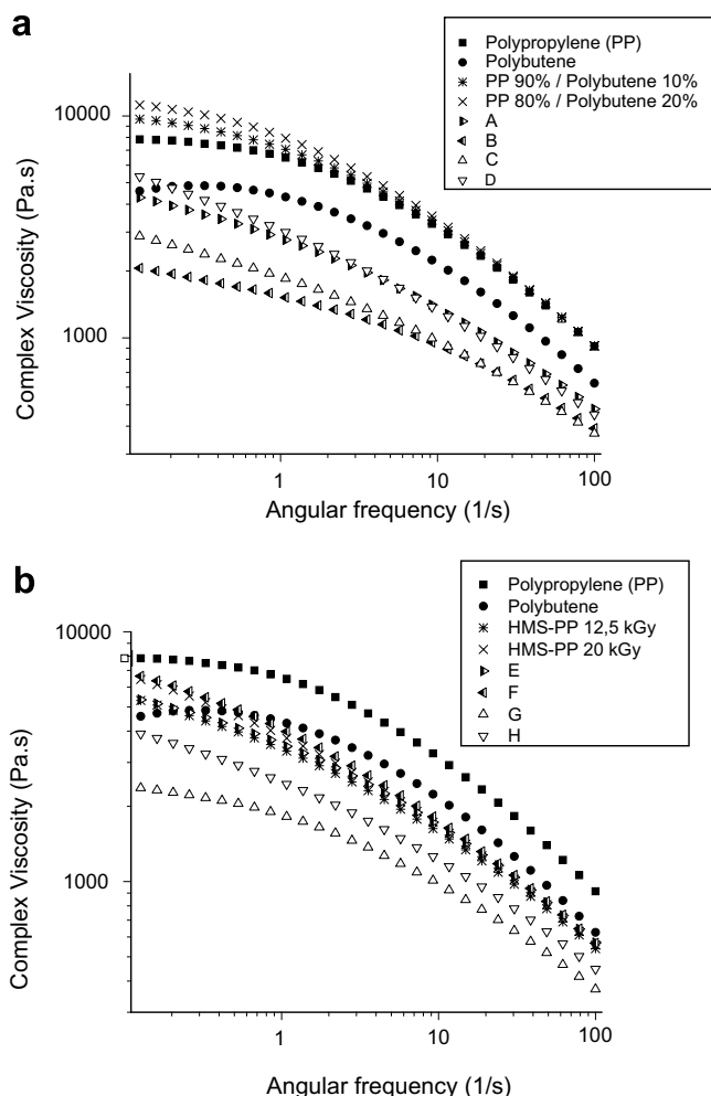
Fig. 2. Complex viscosity as a function of frequency angular for samples: (a) Processed by method 1 and (b) processed by method 2.
