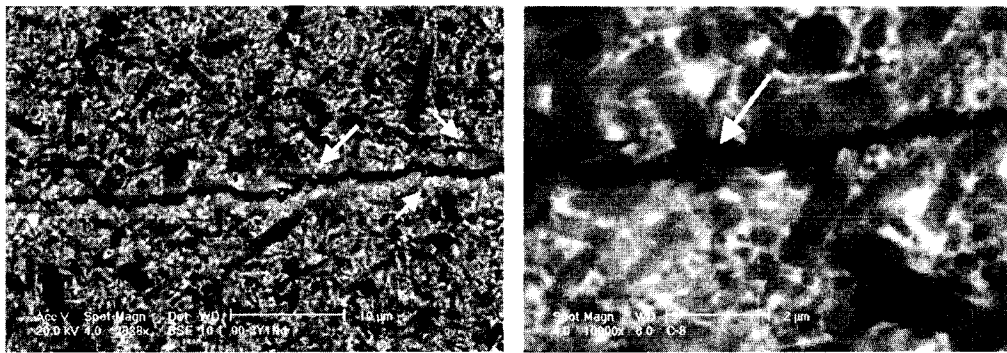
Fig. 3 – Crack propagation profile of \text{Si}_3\text{N}_4 : (a) 90-3Y1Nd and (b) 90-3Y3Nd. Interaction between the crack and the grains.
