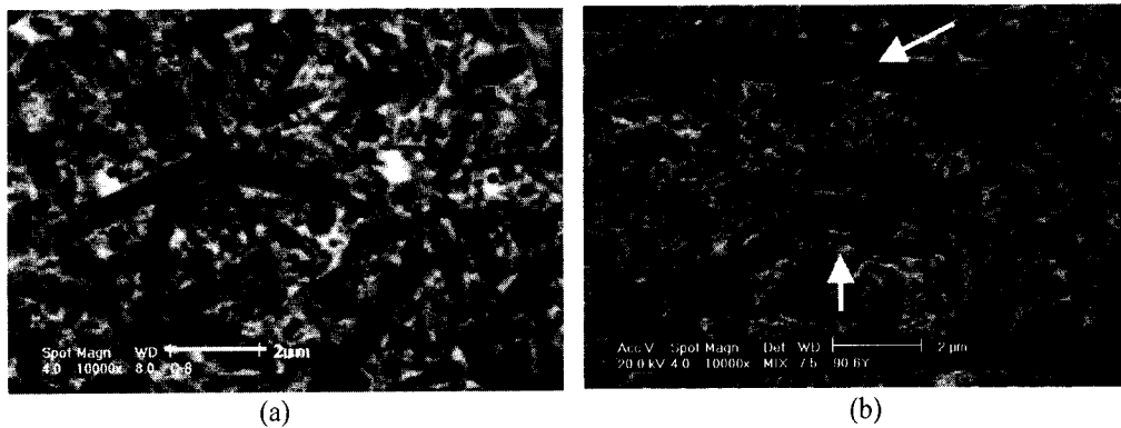
Fig. 2 – Microstructure of samples polished and plasma etched (a) 90-3Y3Nd; (b) 90-6Y.
