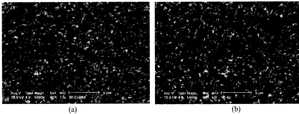
Fig. 1 – Microstructure of samples polished and plasma etched (a) 90-2Y2Nd; (b) 90-4Y.
