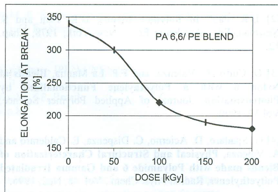
Figure 2. Elongation at break of PA6,6/LLDPE blend as a function of radiation dose.
