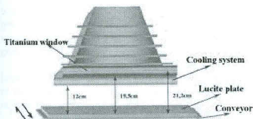
Figure 1. Electron accelerator irradiation parameters [2].
