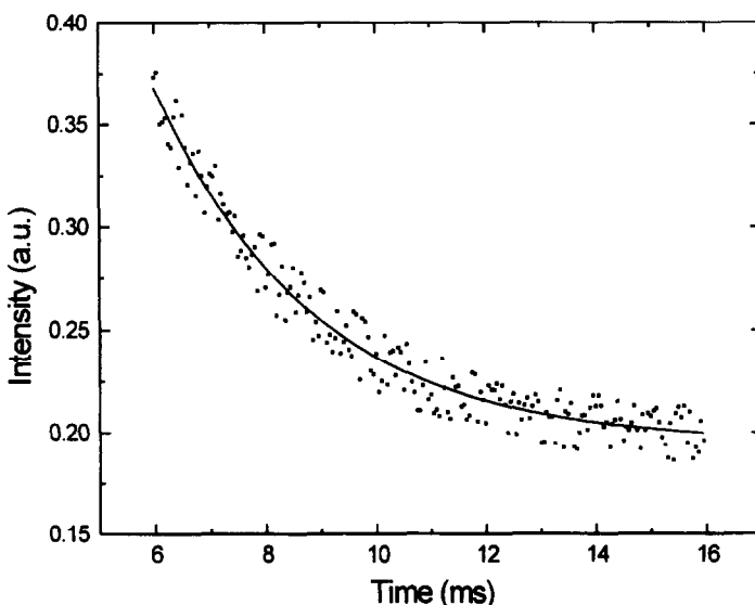
Fig. 3. Temporal behavior of the luminescence intensity when excited by a modulated Kr + ion laser operating at 647 nm. The solid line is the fit of an exponential decay with a constant of 2.8 ms (0.2 ms).
