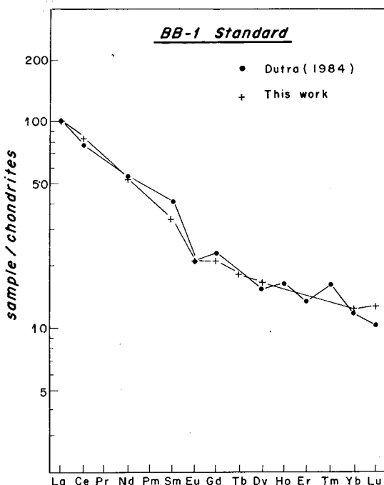
Figure 1 — Chondrite-normalized REE distribution patterns of GB-1 and BB-1 standards. Comparison with literature values.
