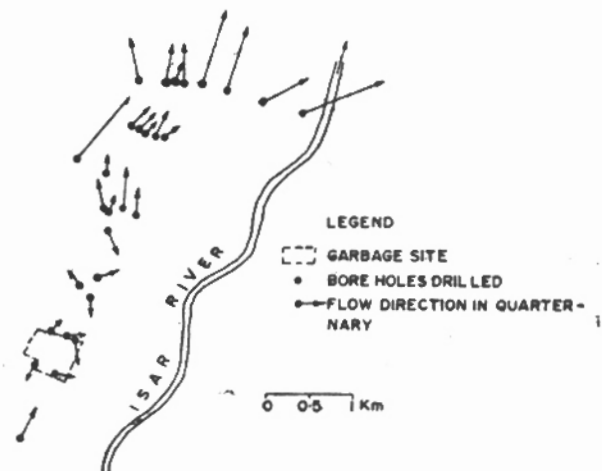
Fig. 8. Ground water flow direction at the garbage disposal site
