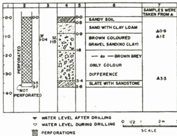
Fig. 4. Typical geological cross-section at borehole X
