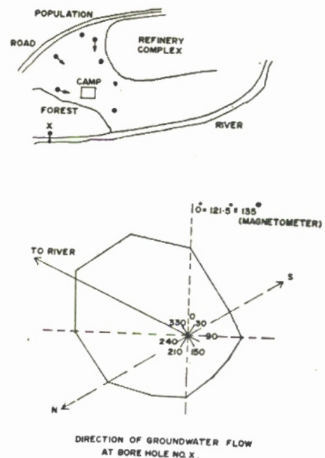
Fig. 3. Plan of boreholes around refinery complex
