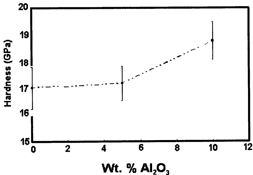
Fig. 1: Variation of WC-Co-hardness as a function of alumina content.
