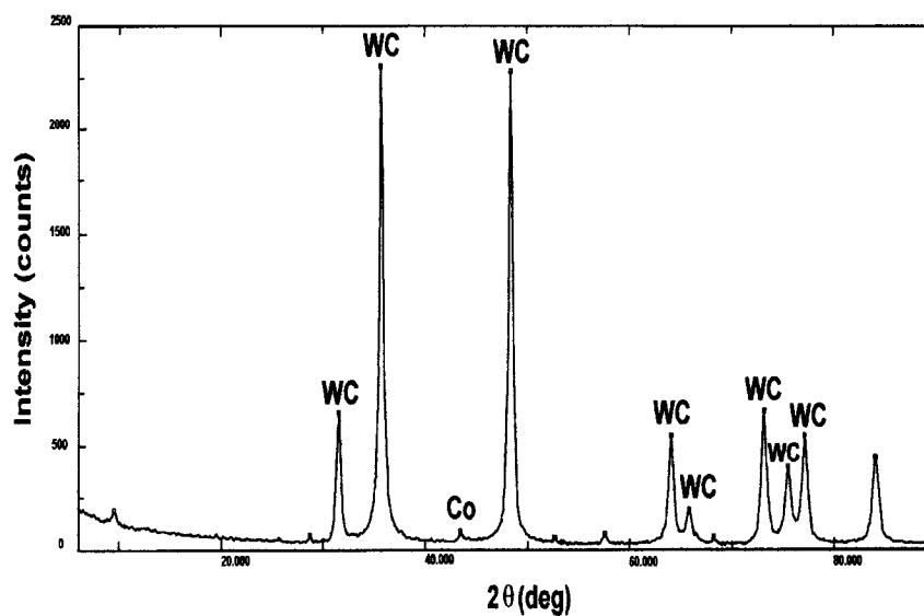
Fig. 4: X-ray diffraction of WC-Co-10 wt.% Al 2 O 3 .
